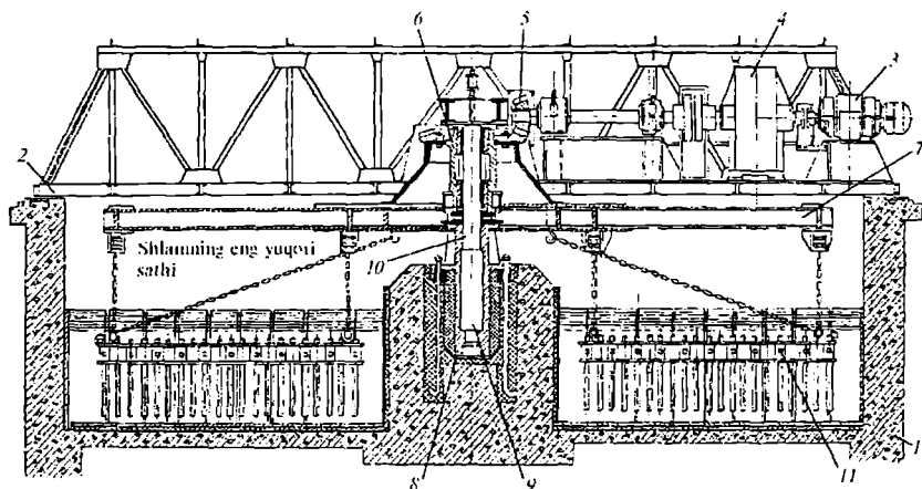
8-rasm. Loychayqatgich.
