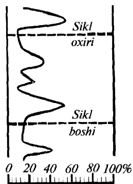
6.15-rasm. Gaz aralashmasining xromatogrammasi.
