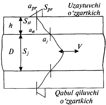
4.20-rasm. Ultratovushli dopler sarfo'lgachigichning ishlash prinsipi.
