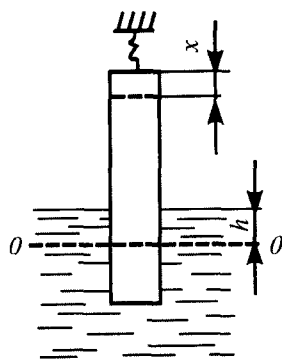
5.4-rasm. O'zgaruvchan botishli silindrik qalqovich siljishining sxemasi.
