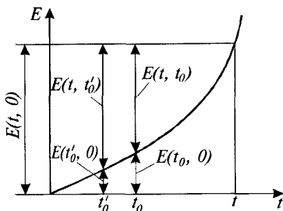
2.4-rasm. Termoelektr termometrning erkin uchlar haroratiga tuzatma kiritish.
