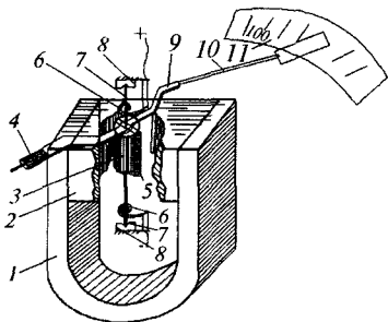
2.8- rasm. Millivoltmetrning tuzilishi.
