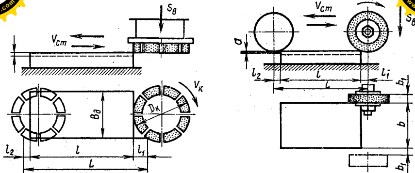
8.5-rasm. Tekis Yuzalarni jilvirlash:
