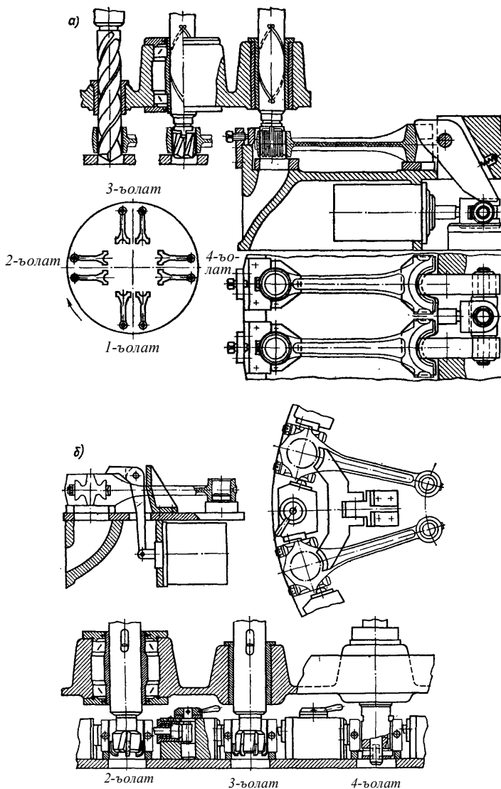
11.3-rasm. SHatun kallaklaridagi teshiklarga ishlov berish: a) porshen kallagidagi teshikka to'rt xolatli olti shpindelli vertikal parmalash yarim avtomatida; b) qopqoq bilan yig'ilgandan so'ng krivoshin kallagidagi teshikka to'rt xolatli olti shpindelli vertikal parmalab-yo'nib kengaytirish dastgohida
