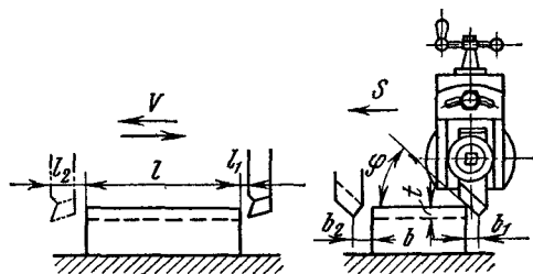
8.1-rasm. Tekis Yuzalarni randalash a) bo'ylama, b) ko'ndalang randalash.
