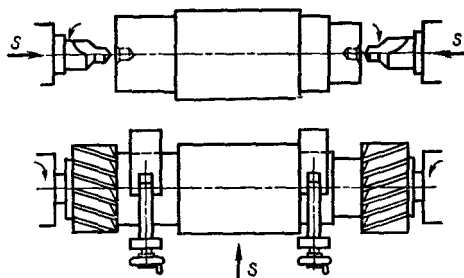
9.4-rasm. Frezerlash-markazlash dastgohlarida ishlov berish.
