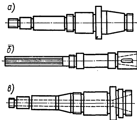
9.1-rasm. Metall kesish dastgohlarida shpindellarning tuzilishi:
