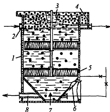
39-rasm. Pnevmatik flotatsiya mashinasi \Phi\Pi-100 :
