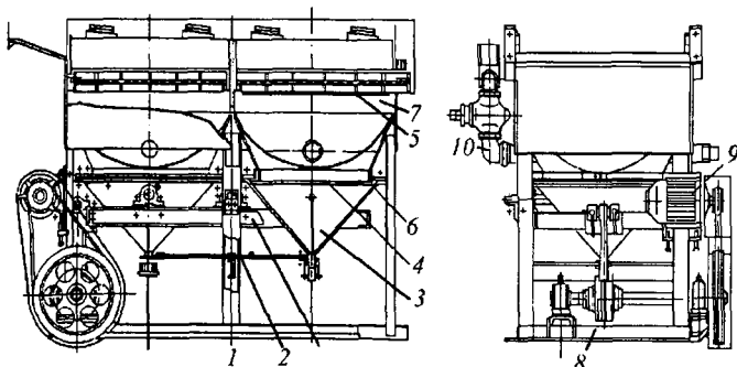
27- rasm. Diafragmali cho'ktirish mashinasi MOД-2. 1-prujinalanuvchi resor; 2-3- voronka; 4-gardish; 5-panjara; 6-manjet; 7-korpus; 8-shatun-ekssen 10-kollektor.
