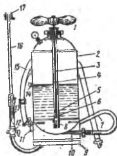
2.70-rasm. Avtomaksning sxematik ko‘rinishi: 1- shtok dastasi, 2-rezervuar, 3- nasos silindri, 4- porshen shtoki, 5- porshen buferi, 6- porshen, 7-shlang, 8- haydaydigan klapan, 9- karkas, 10- shtutser, 11- tasma, 12-bekitadigan kran, 13- filtr, 14- kontrol sath probkasi, 15- kamar, 16-chiqaruvchi metall naycha, 17-qo‘sh rojokli changlatgich
