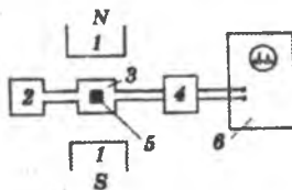
2.47-rasm. EPR spektrometrining sxematik ko'rinishi
