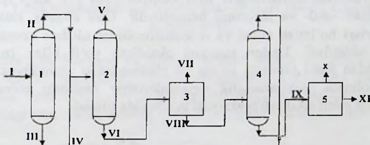
11-rasm. Ksilol fraksiyasini individual uglevodorodlarga ajratish prinsipl sxemasi:
