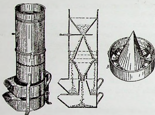
30-rasm. Gusev bo'lgichi:
