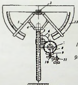
47- rasm. G-2 markali gibkomer:
