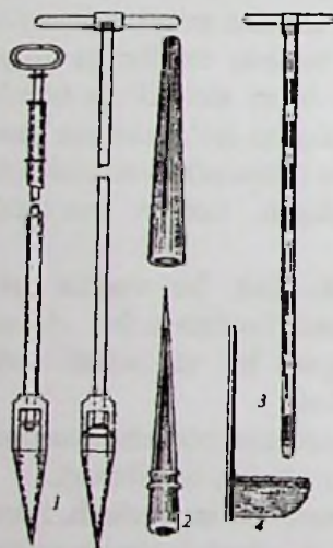
26- rasm. Don shuplari va cho'mich: 1-vagon konus shuplari; 2-qop shupi; 3-silindr shup; 4-cho'mich.
