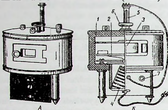
32-rasm. SESH-3M elektr quritish javoni:
