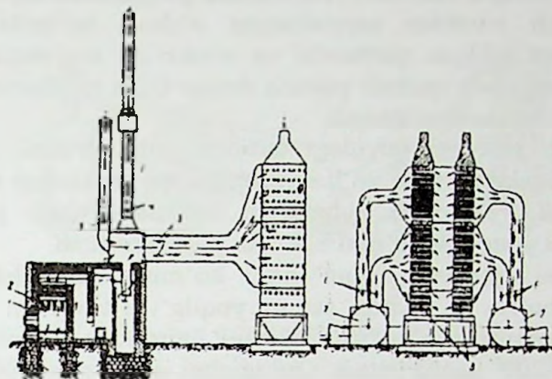
38-rasm. SZSH-8 don qurtgichi (chizmasi):
