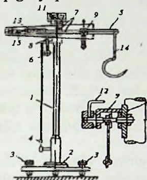
46- rasm. Tola namunasini tayyorlaydigan PO-2 asbobi:
