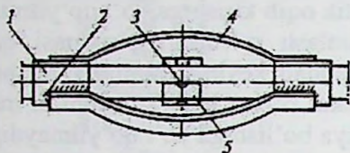
5.5-rasm. Prujinali markazlagich:
