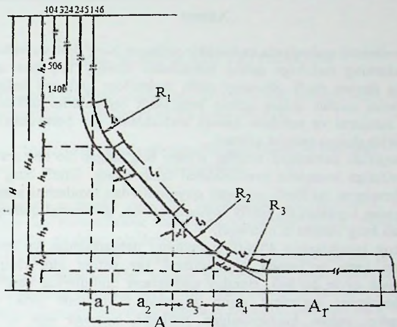
9.2-rasm. Gorizontal quduqning hisobiy profili
