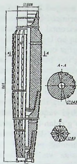
17.5-rasm. Universal rayber-frez RFU-168
