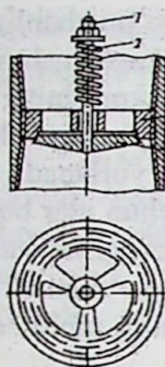
5.2-rasm. Likopchali klapan:
