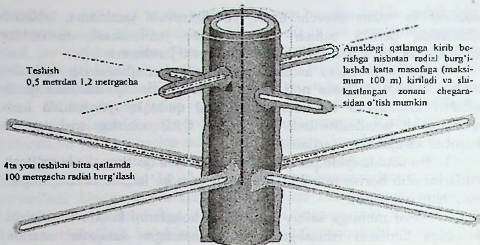
20.8-rasm. Radial burg'ilashni ikki qatlamda olib borish
