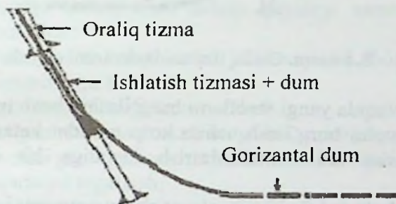
8.3-rasm. Ishlatish tizmasi–dumda derazani ochish
