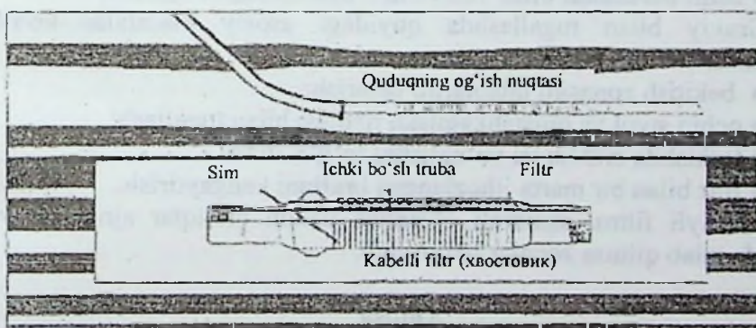
14.10-rasm. Gorizontaal quduq – urma kirgizmali filtrlı xvostovik
