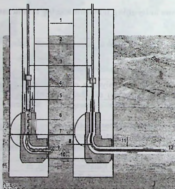
20.9-rasm. Qatlamni radial ochish sxemasi
