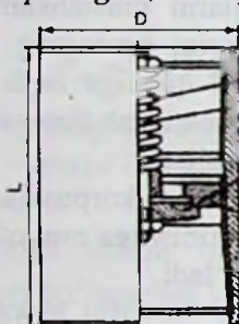
5.3-rasm. Likopchali teskari klapan
