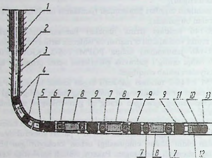
13.4-rasm. Gorizontal quduq tugallangandan keyin uni ishlatishga tayyorlash:
