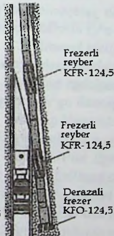
17.3-rasm. Yon stvol derazasini qirg'ishning ketma-ketligi
