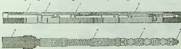
20.5 -rasm. Radial burg'ilash uchun frezerlash jamlanmasi:
