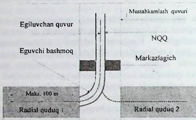
20.1-rasm. Radial quduqni burg'ilash jarayonini olib borish tartibi
