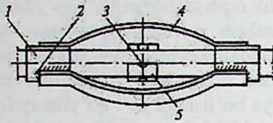
5.5-rasm. Prujinali markazlagich:
