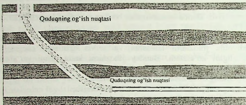
14.6-rasm. Gorizontal quduq – sementlash «xvostovigi» bilan mustahkamlangan
