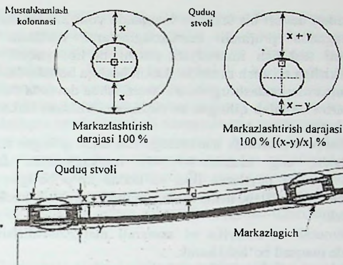
14.9-rasm. Mustahkamlash tizmasini markazlashtirish darajasi
