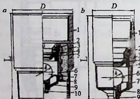
5.4-rasm. Sementlashda qo'llaniladigan drosselli teskari klapan:
