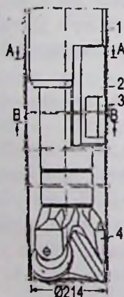
1.10-rasm. Elastik og'dirgich: 1-turbobur; 2-og'dirgich; 3-rezinali reszor; 4-burg'i.
