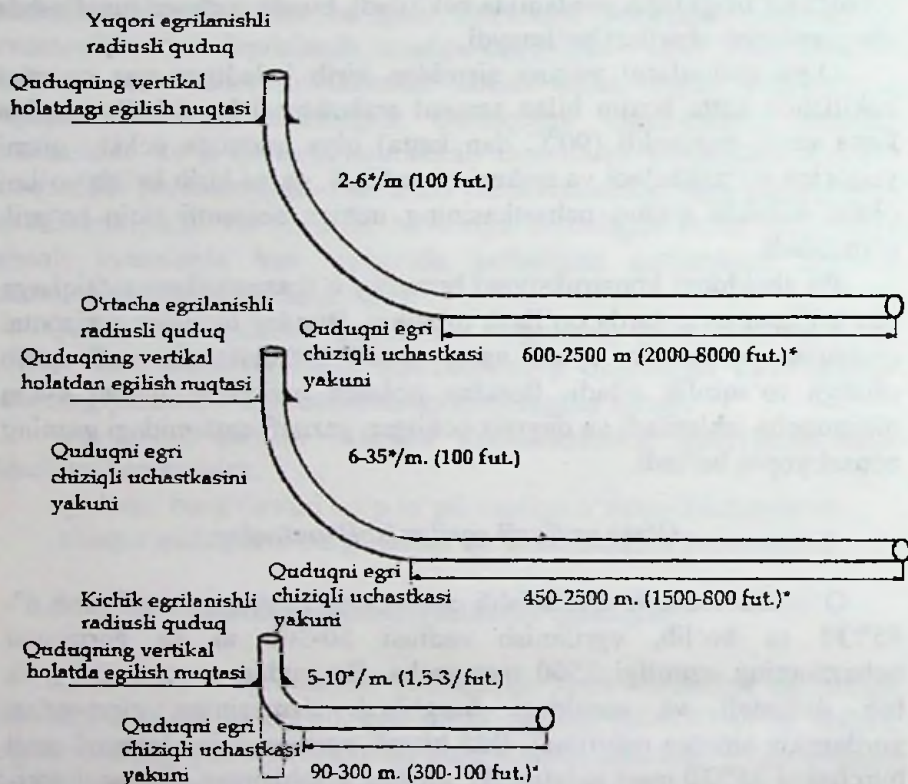
6.4-rasm. Quduqlarni tugallashni kichik, o'rtacha va katta radiusli egrilanish shakllari
