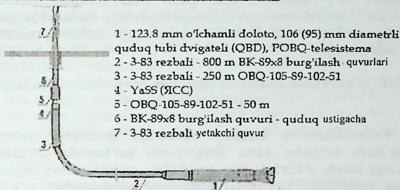
6.7-rasm. Burg'ilash tizmasining osti jamlanmasi
