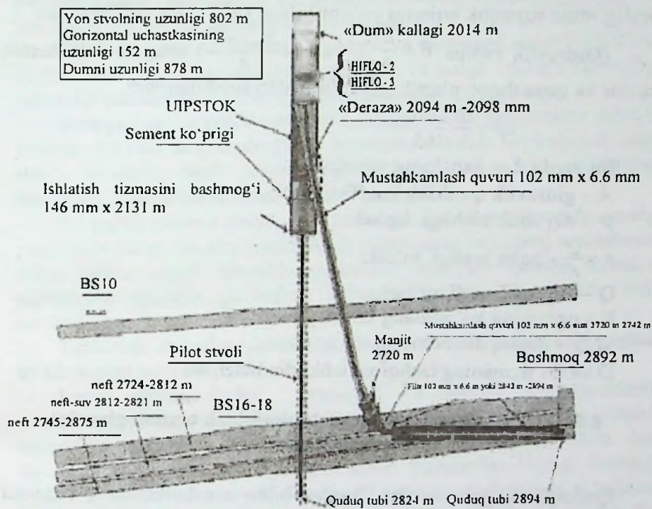
8.6-rasm. Qudug yon stvolining gorizontal profili
