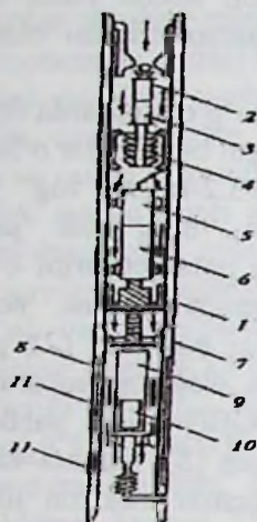
13.2-rasm. RGD armaturasiining prinsipial sxemasi:
