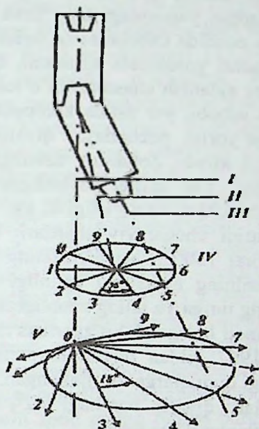
13.1-rasm. Qiyalik burchakning o'zgarish sxemasi:
