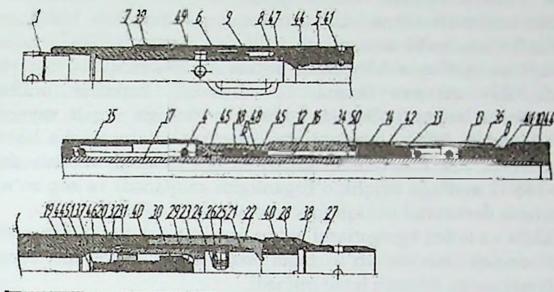
13.10-rasm. MSP-146S2 turidagi o'tuv sementlash muftasi
