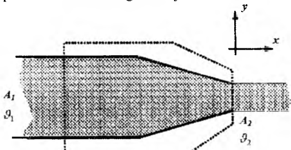
3.25.4-rasm. Quvur soplodagi kuchlar
