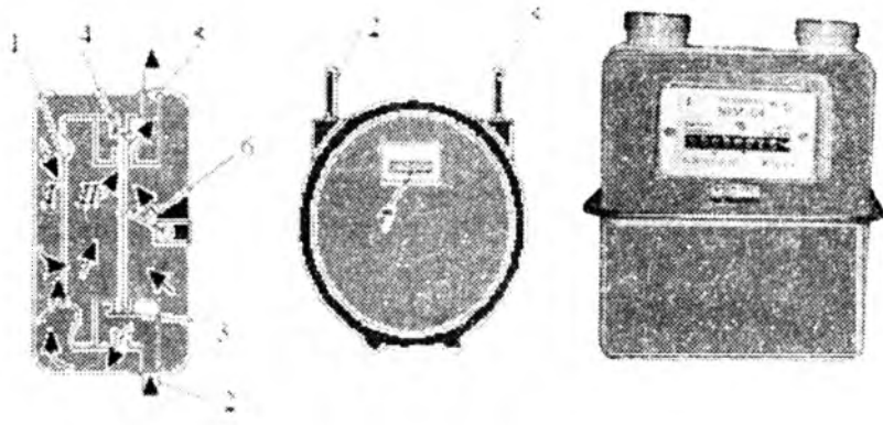
2.26.13-rasm. GKF tipidagi diafragmali hisoblagich
