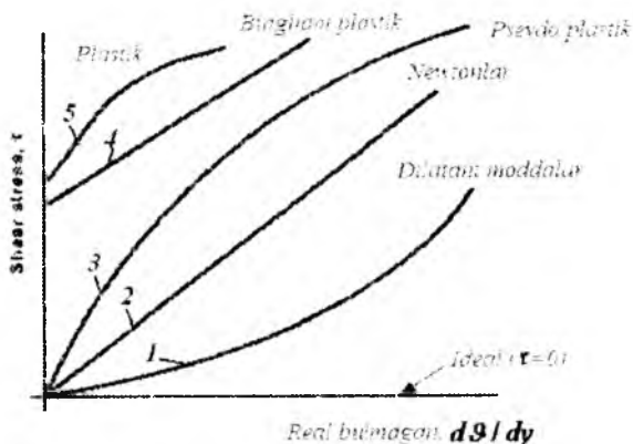
2.17.2-rasm. Siljish deformatsiyasi tezligiga bog'liq siljish d\theta / dy
