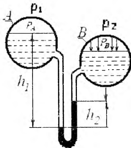
2.26.3-rasm. Differentsial manometr
