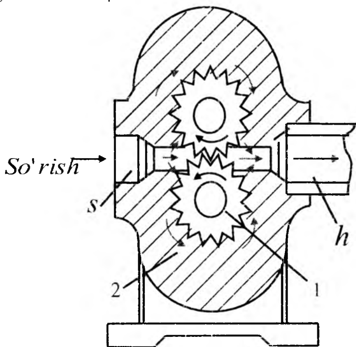
8.15.1-rasm . Shesterniyali nasos
