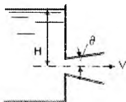
7.5.5-rasm. Tashqi silindrik kengayuvchi naycha
