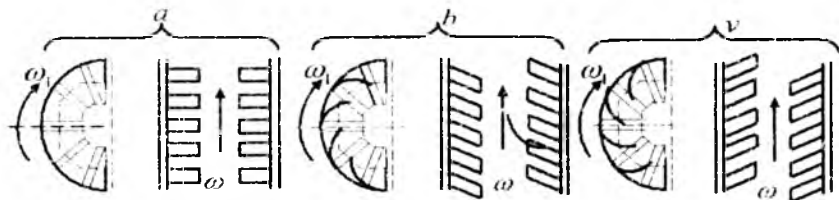
8.16.2-rasm. Radial kurakli ish g'ildiraklari.
