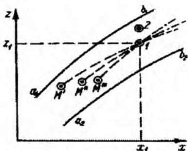
3.2.3-rasm. Suyuqlik zarrachalarining beqaror harakati.
