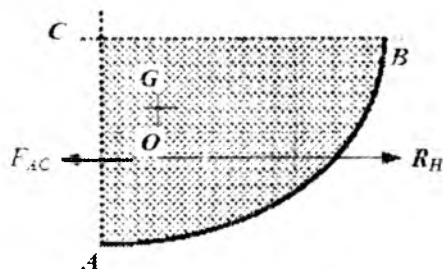
2.7.2-rasm. Cho'kgan egri AC , F_{AC} gorizontal kuch
