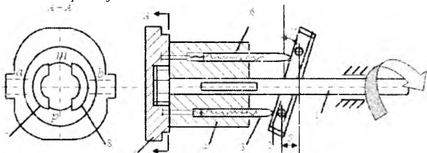
8.15.3-rasm. Aksial porshenli nasos sxemasi
