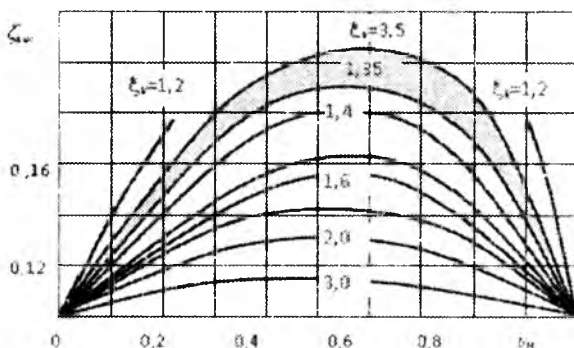
7.7.6 –rasm. Tiklanish farqini aniqlash uchun grafik
