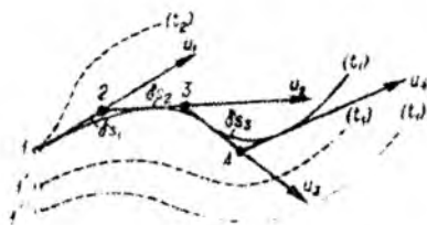
3.2.5-rasn. Beqaror harakatdagi oqim chizig'i.
