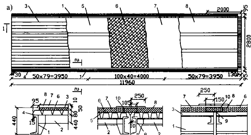
14.1-rasm. Yengillashtirilgan yopma plita:
