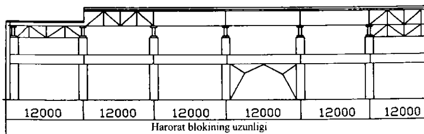
8.18-rasm. Tik bog'lamlar:
