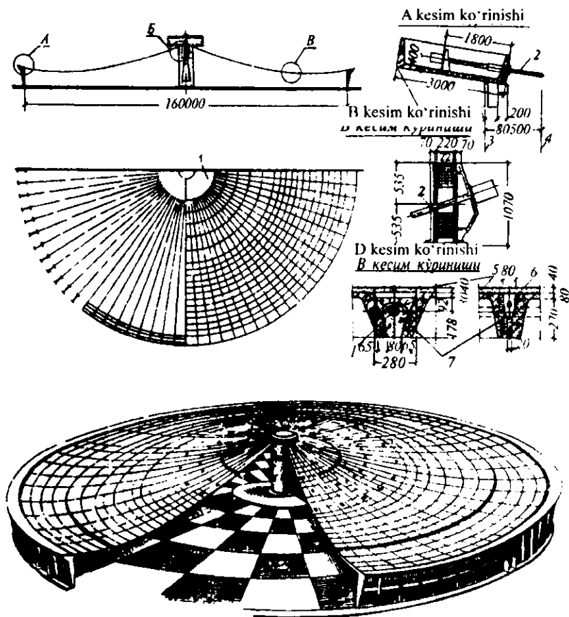
8.16-rasm. Markaziy tayanchli osma vantalar:
