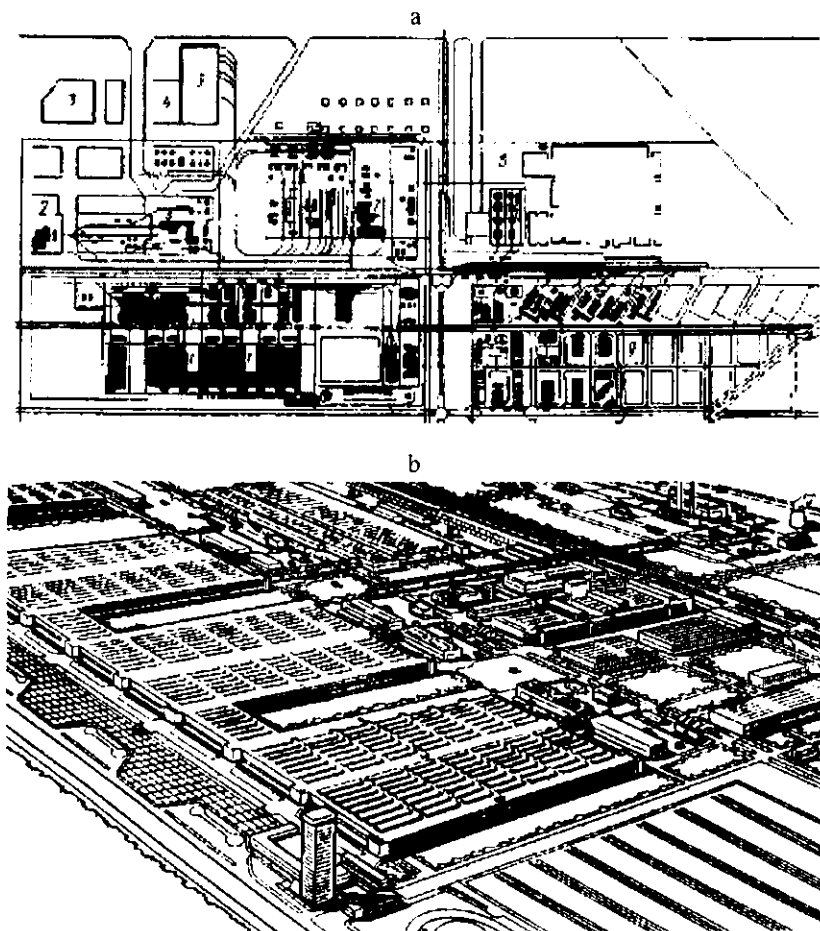
4.1-rasm. Yengil avtomobillar yirik zavodining bosh rejasi:
