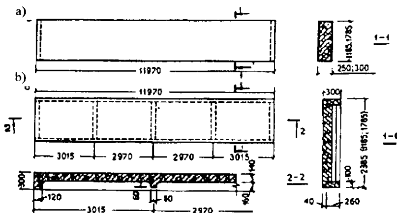
11.4-rasm. Isitiladigan binolarning 12 m li devor panellari:
