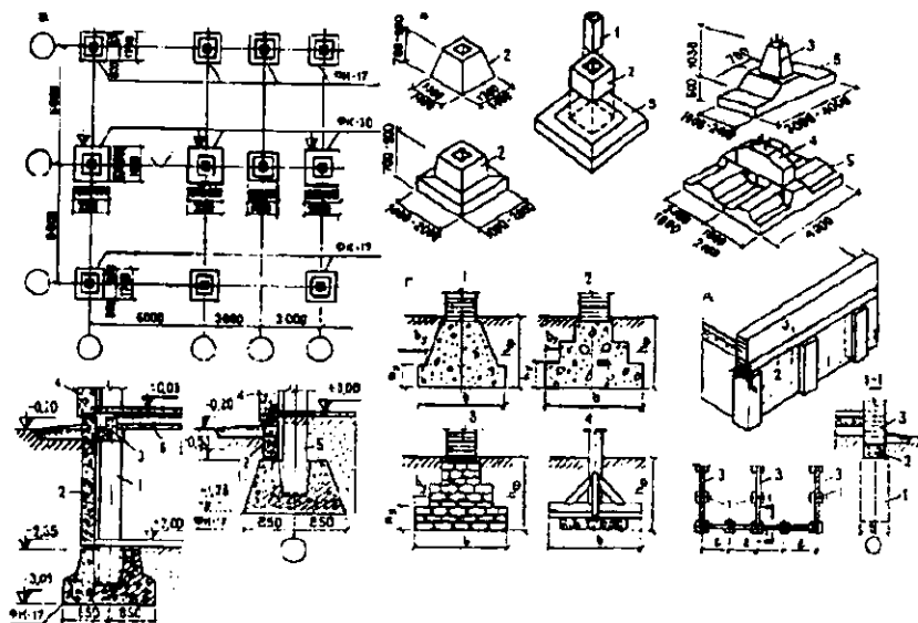
12.7-rasm. Ustunsimon poydevorlar:
