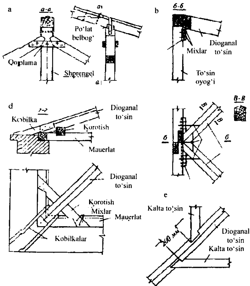
17.5-rasm. Chordoq to'sinlarining detallari: a–diagonal to'sinning shprengelga tayanish birikmasi; b–diagonal to'sinning to'singa tayanishi; d–diagonal to'sinning mauerlatga tayanishi; e–kalta to'sinlarning diagonal to'singa birikishi
