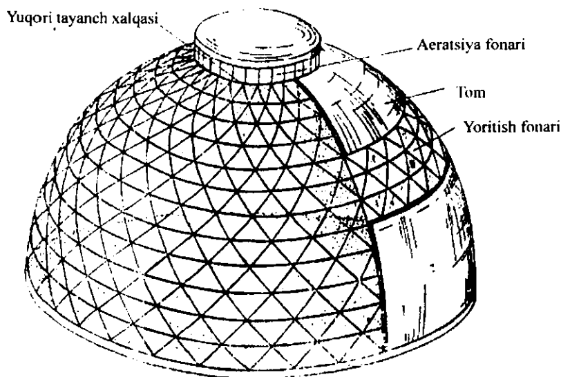
27.5-rasm. To'rtli gumbaz chizmasi
