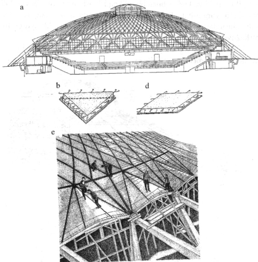
27.4-rasm. Rimdagi kichik olimpiya arenasining quyma-yig'ma yopma gumbazi: a–qirqim; b, d–yopmaning yig'ma armosement elementlari; e–gumbaz montaji
