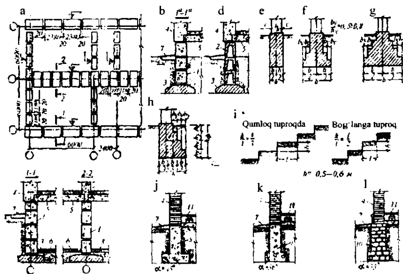
12.5 - rasm. Tasmasimon poydevorlar:
