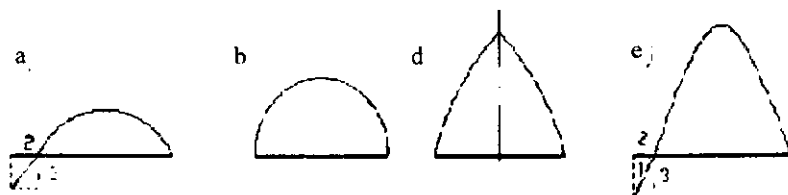
25.3-rasm. Arkalarning sxemalari:
