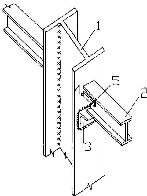
24.7-rasm. Po'lat rigelining po'lat ustunga tayanishi: 1—ustun; 2—rigel; 3—tayanach burchak «stolik»; 4—plastina; 5—bolt
