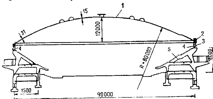
27.2-rasm. Sport zalining temir-beton gumbazli qoplamasi:
