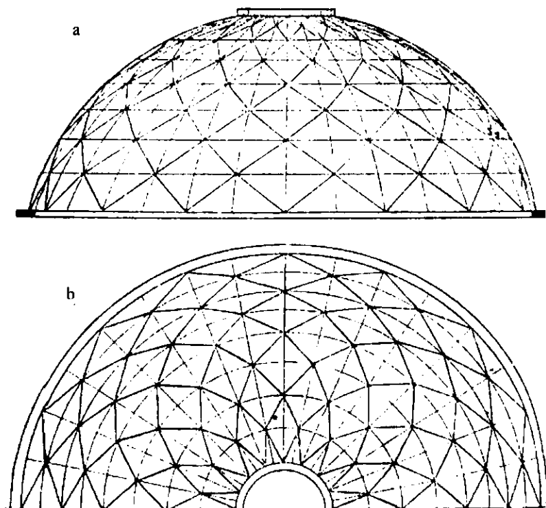
27.7-rasm. Geodezik gumbaz chizmasi: a—qirgim; b—rejasi
