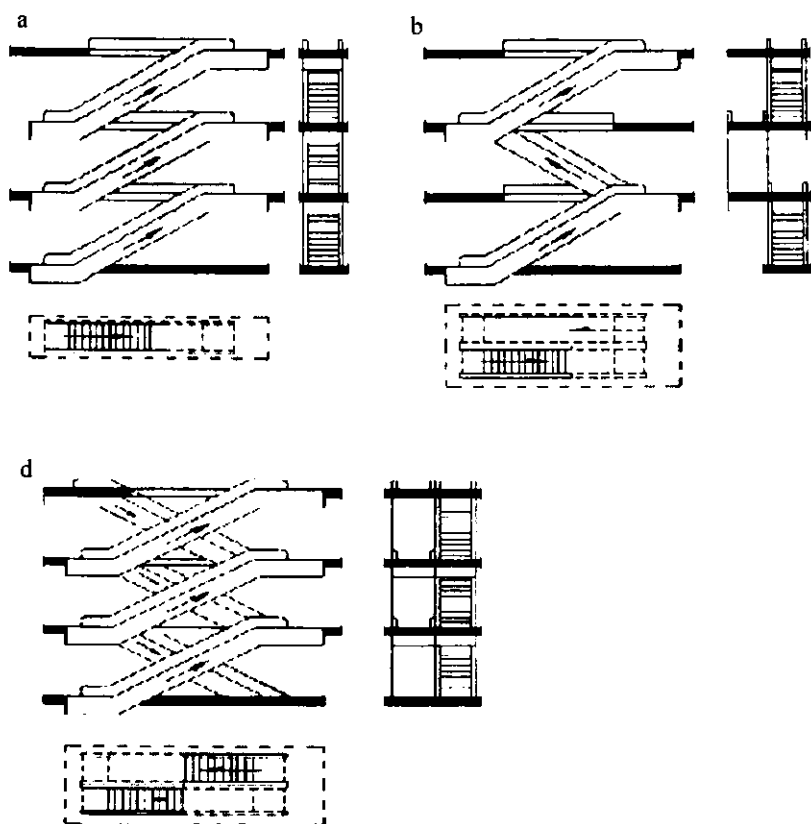
22.16-rasm. Eskalator chizmalari: a- parallel marshli; b- ketma-ket; d- kesishuvli
