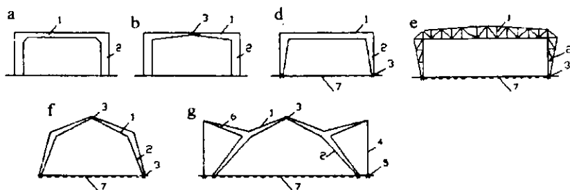
25.2-rasm. Katta prolyotli tomalar ramalarining sxemalari:
