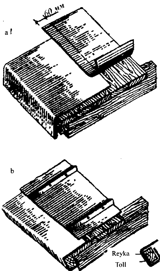
17.8- rasm. O'rama toldan bajarilgan tomlar: a–ustma-ust qirraga parallel; b–uchburchak reyka yordamida
