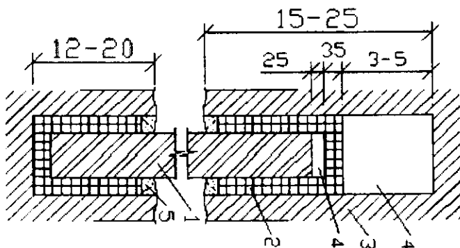
30.2-rasm. Aluminiy vitrajlarda shishalarni qotirish:
