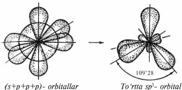
3.10- rasm. Valent orbitallarning sp - gibrirlanishi.
