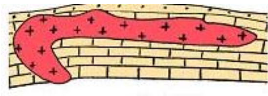
3.19-rasm. Garpolit.
