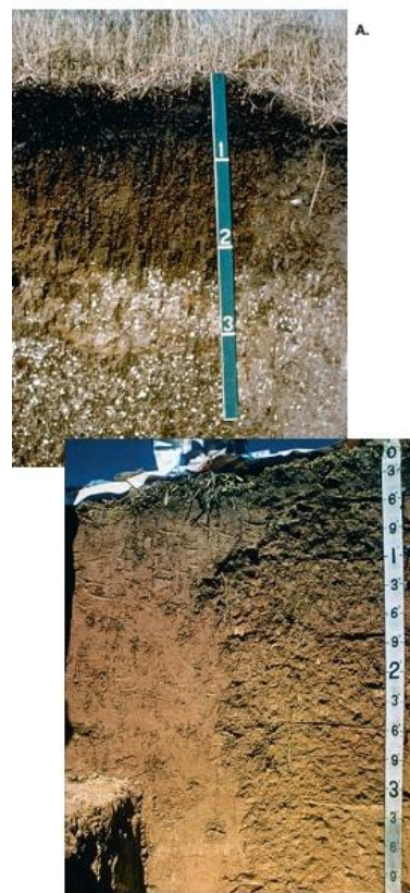
7.11-rasm. Tuproq nurashi.
