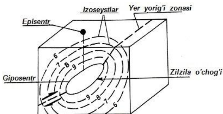
13.1-rasm. Zilzila o'chog'ining tuzilish sxemasi
