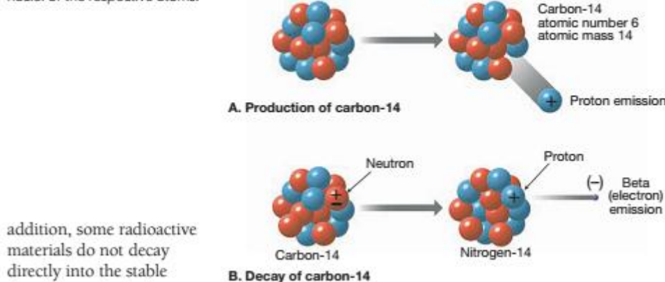
FIGURE 18.18 A. Production and B. decay of carbon-14. These sketches represent the nuclei of the respective atoms.
