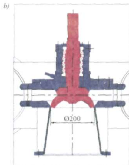
39-rasm. 20 ПpД parrakli diagonal turbinaning ishchi holatidagi ko'rinishi (a) o'rnatilish sxemasi va (b).
