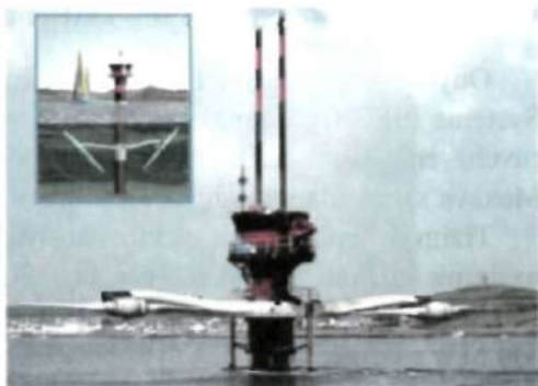
15-rasm. Suv sathining ko'tarilib-tushish prinsipi asosida ishlaydigan eng katta turbina.
