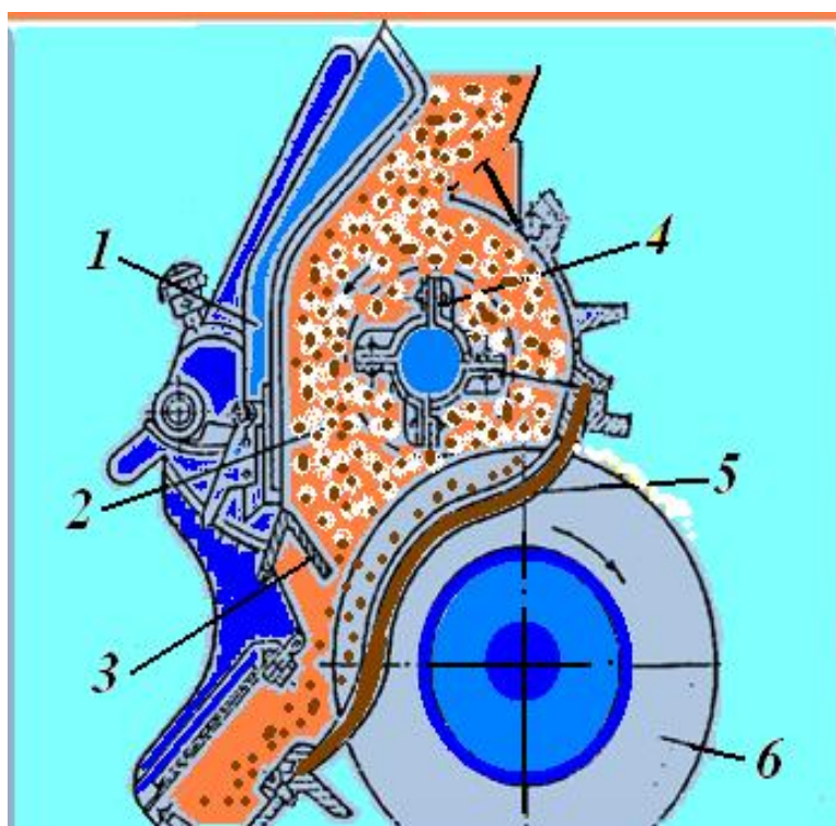
70-rasm. Linterning to'zitgich bilan arra orasining o'zaro ta'sir sxemasi
