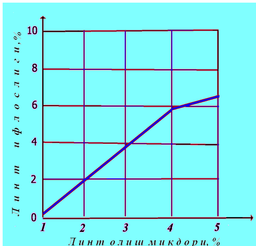
72-rasm. Lint iflosligining lint olish miqdoriga ta'siri
