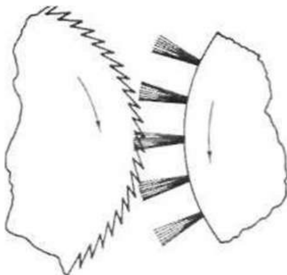
56-rasm. Cho'tkali barabanning arra silindr tishida tolani ajratib olishi
