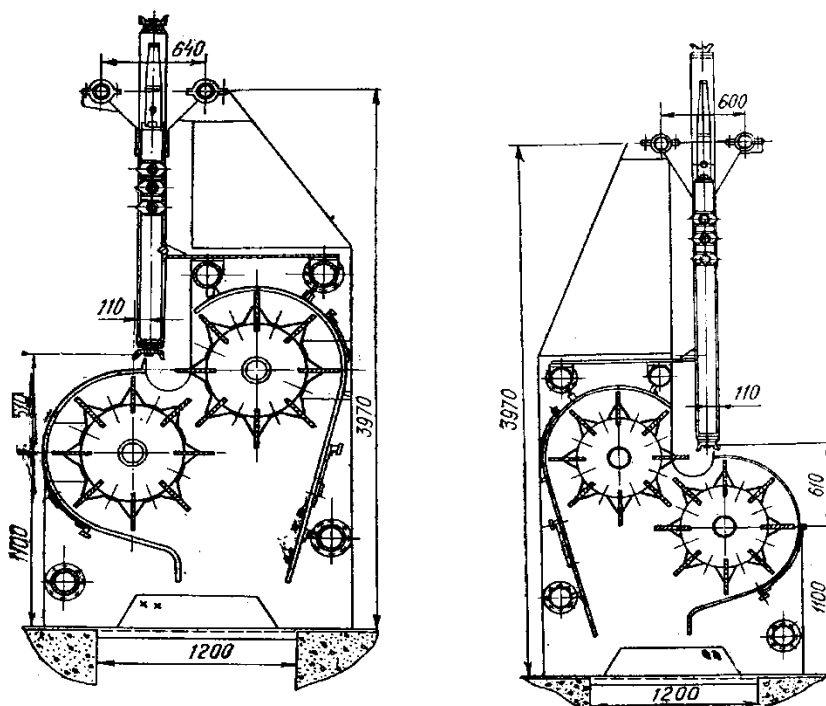
89-Rasm. AJT rusumli titish-yuvish mashinasi
