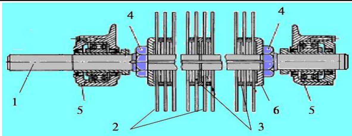
48-rasm. Arrali silindrning tuzilishi
