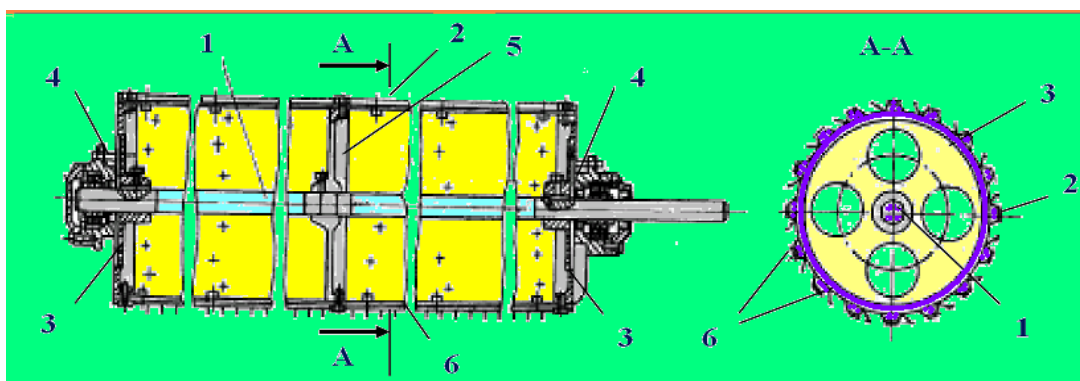
63-rasm. Ignali baraban
