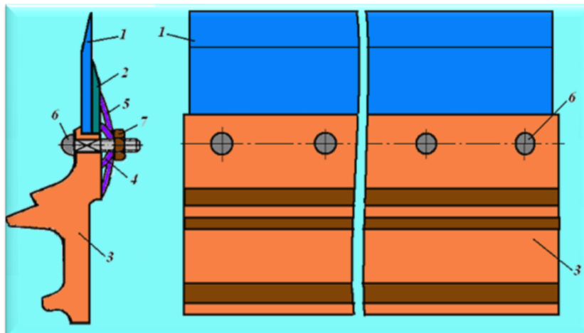
64-rasm. Valikli jinning qo'zg'almas pichog'i 1-Pichoq; 2-nakladka; 3-deka; 4- skobalar; 5-prujina; 6-gayka; 7- bolt.
