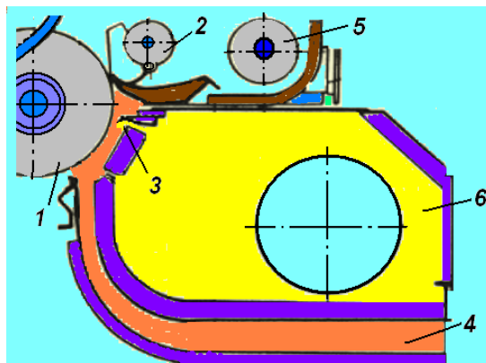
52-rasm. Tolani arra tishlaridan ajratuvchi moslamalar sxemasi
