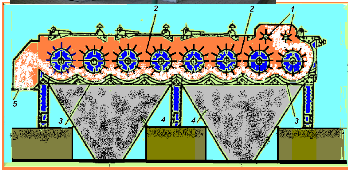
35- rasm. 1XK paxta tozalash mashinasining sxemasi
