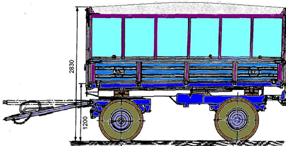
12-rasm. Chigitli paxtani tashishda foydalanidigan 2PTS-4-793 rusumli tirkaladigan arava
