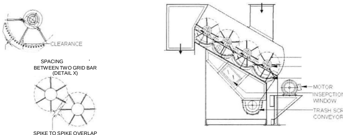
38-Rasm. Qiya tozalagich sxemasi
