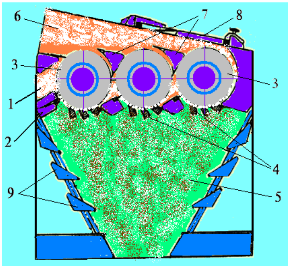
75-rasm. 1-BII rusumli tola tozalagichning texnologik jarayon sxemasi
