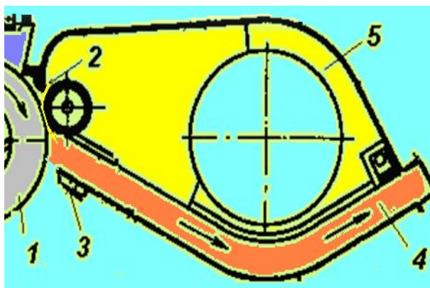
52-rasm. Tolani arra tishlaridan ajratuvchi moslamalar sxemasi
