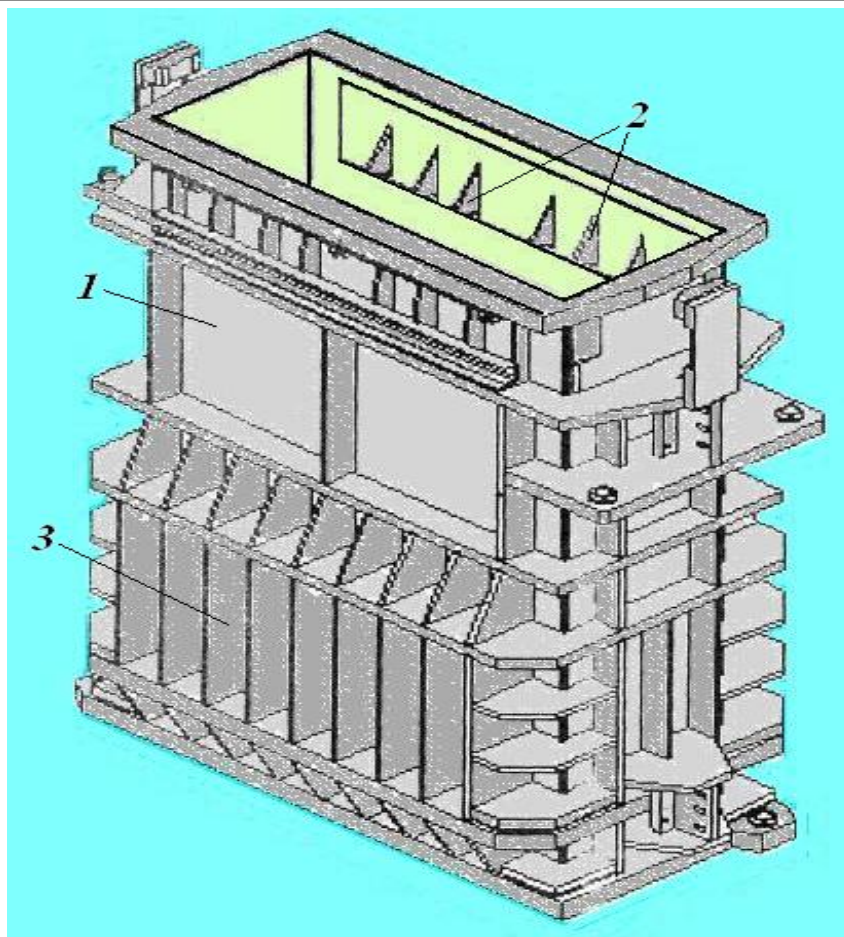
68-rasm. Press-kameranin tashqi ko'rinishi 1-press-yashik; 2-tola ushlagichlar; 3-press-kamera.
