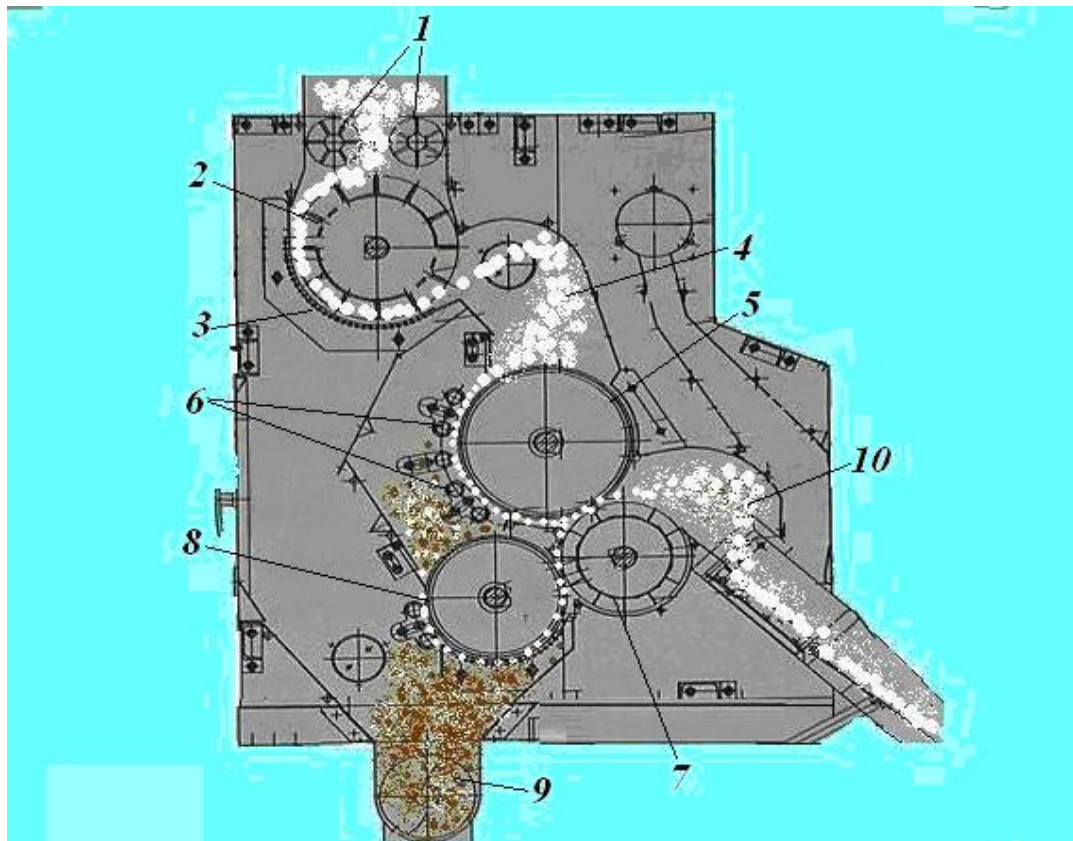
65-Rasm. - MYJ 118 rusumli jin ta'minlagichi
