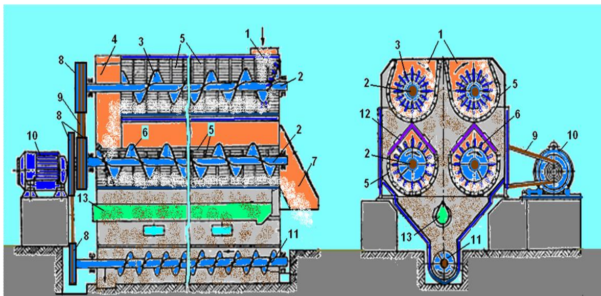
39- rasm. 6A-12M rusumli shnekli paxta tozalash
