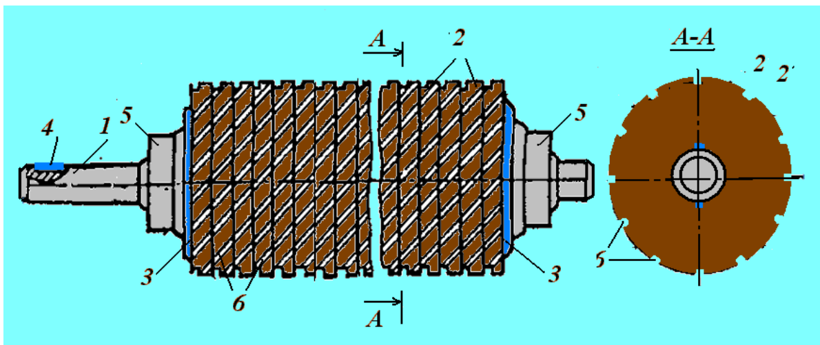
60-rasm. Valikli jinning ishchi barabani
