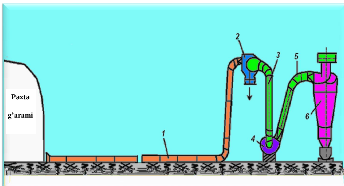
15-rasm. Pnevмотransport qurilmasi
