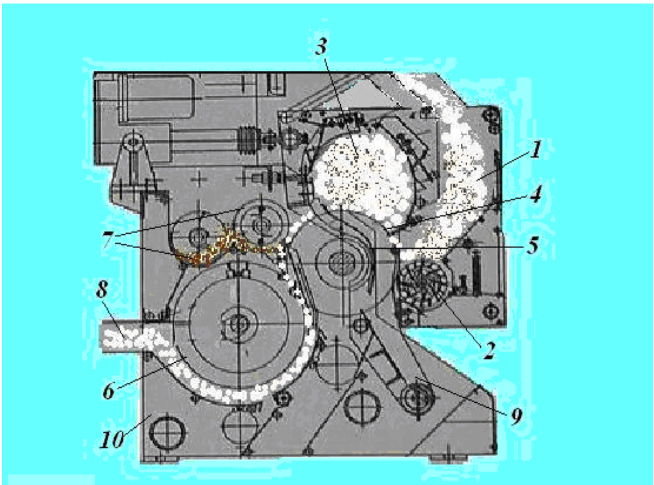
66-Rasm. MYJ – 118 rusumli arrali jin
