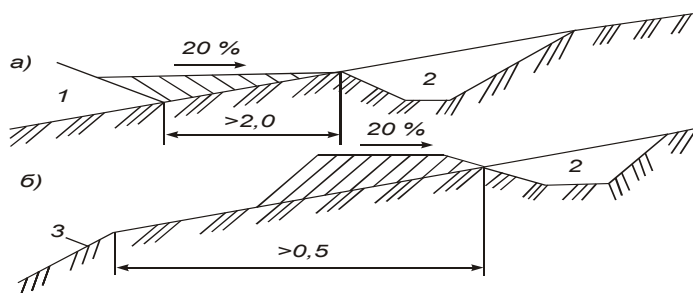
18-rasm. Tog' yon bag'ir ariqchalari
