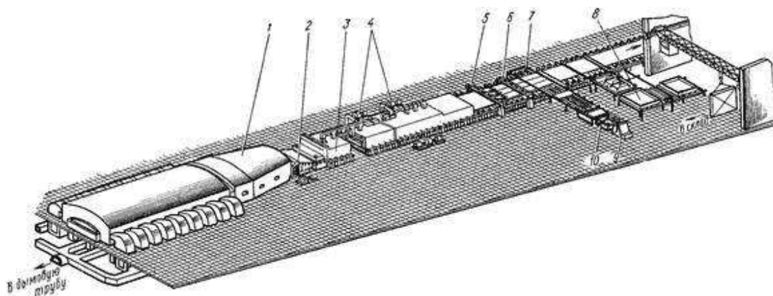
Rasm.2. Pishirish usuli. Nomerlarni kodlash: 1 - hammom pechi, 2 - prokatlash mashinasi, 3 - tavlanadigan pech, 4 - gaz aylanma tizimi, 5 - uzun kesish mexanikasi, 9 - pishirgich, 7 – yo'nlitirgich, 8 - qadoqlash uchun stol, 9 - shisha uchun kran, 10 - shisha uchun shisha
