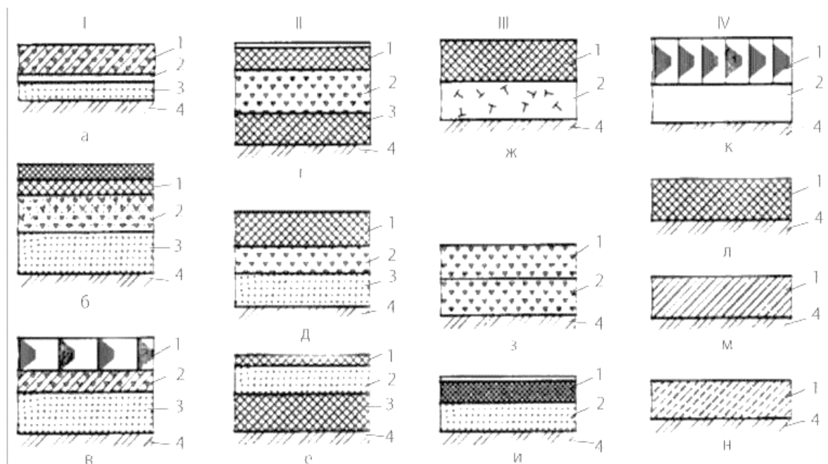
5.12-rasm. I(a-v), II(g-e), III(j-i), IV(k-n) toifali avtomobil yo'llari uchun to'shamaning konstruksion qatlamlari:
