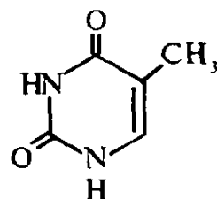
timin
