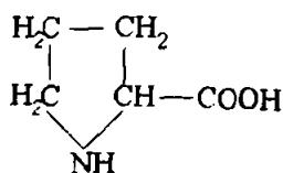
Prolin
