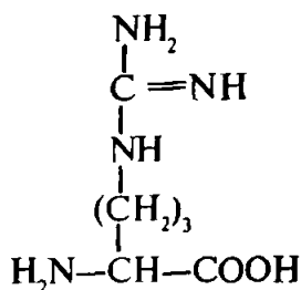
Arginin
