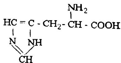
Gistidin
