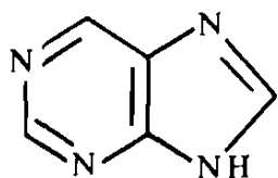
Purin
