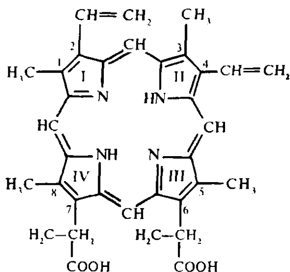
Protopofirin
