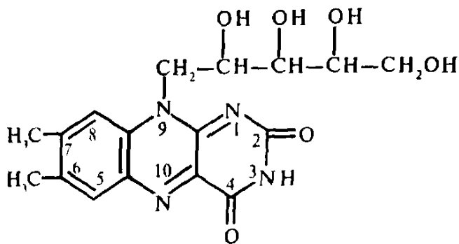
riboflavin
