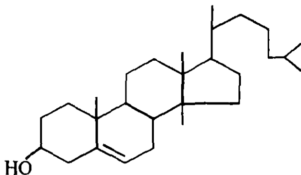
Xolesterin ( C_{27} )
