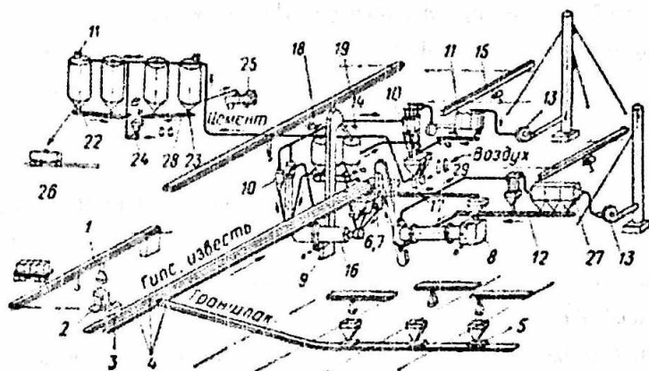
9.2-rasm. Ohak-shlak sement ishlab chiqarish texnologik sxemasi
