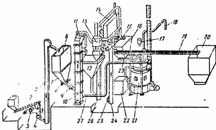
2.7-rasm. Pishirish qozonida qurilish gipsini olish chizmasi
