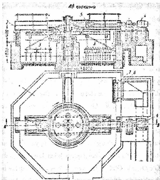
5.3- rasm Gilqorgich- chayqatkich.
