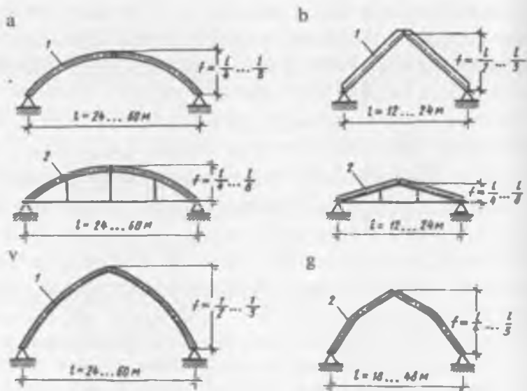
18.7-rasm. Yelimlangan ravoqlar: a – segmentsimon; b – uchburchakli; v – yoysimon; g – siniq yoysimon; 1 – tortqisiz; 2 – tortqilli
