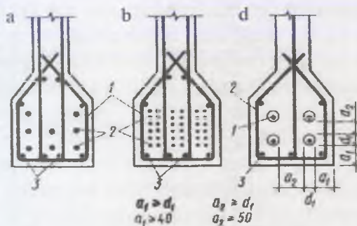
11.6-rasm. Oldindan zo'riqtirilgan to'sinning cho'zilgan zonasini armaturalash:
