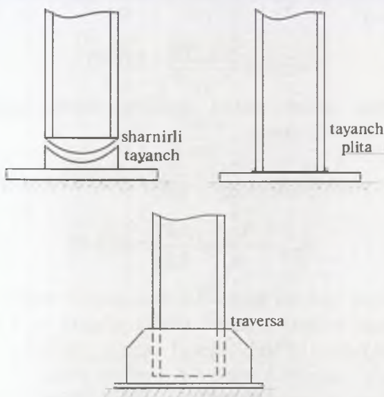
6.3-rasm. Ustun asoslari
