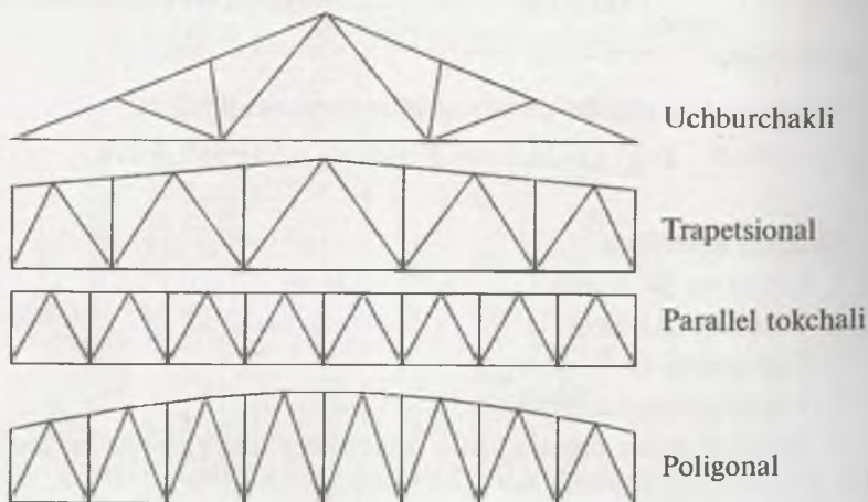
7.1-rasm. Fermalar
