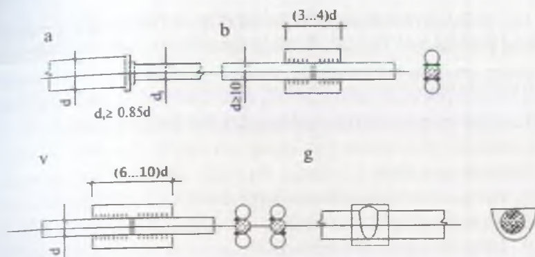
8.3-rasm. Armaturani payvandlashi:
