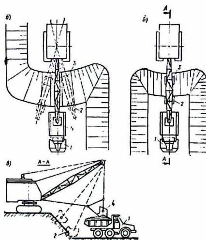
3.7-rasm. Draglayn yordamida zaboyni ishlash sxemasi:
