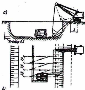
4.2-rasm. Buldozer yordamida to'kmalar barpo qilish:
