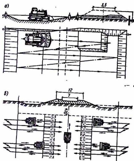
4.2-rasm. Buldozer yordamida to'kmalar barpo qilish:
