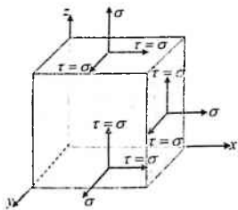
4.20-chizma. Hajmiy kuchlanish holatidagi parallelepiped.
