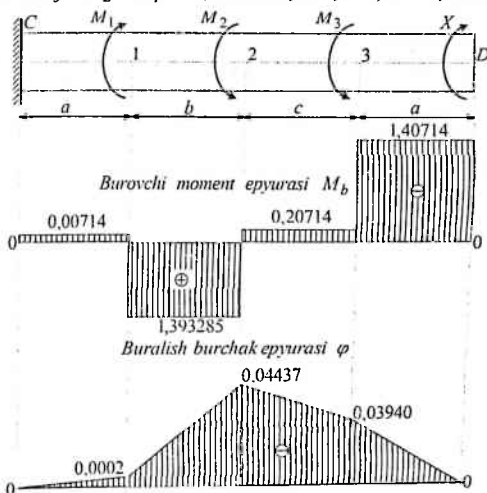
7.9-chizma. Buruvchi moment va buralish burchak epyuralari
