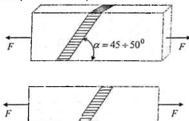
5.14-chizma. Qiya chokli payvandlash
