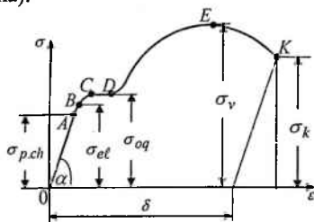
3.4-chizma. Po'lat 3 materialining shartli cho'zilish diagrammasi
