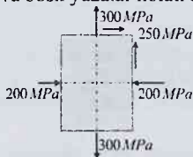
2.33-chizma. Tekis kuchlanish holatidagi element
