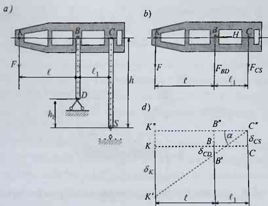
2.28-chizma. Yuk ko'tarish kran modeli
