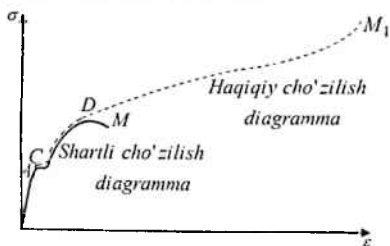
3.12-chizma. Po'lat 3 materialining shartli cho'zilish diagrammasi
