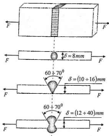
5.13-chizma. Polosani uchma-uch payvandlash
