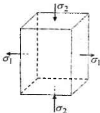
4.26-chizma. Tekis kuchlanganlik holatidagi parallelepiped.
