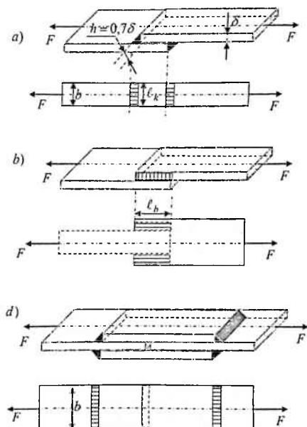
5.15-chizma. Polosani ustma-ust payvandlash
