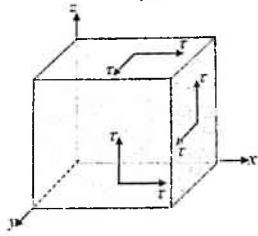
4.21-chizma. Tekis kuchlanish holatidagi parallelepiped.
