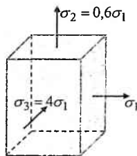
4.25-chizma. Parallelepipedga turli ishorali kuchlanishlar ta'siri
