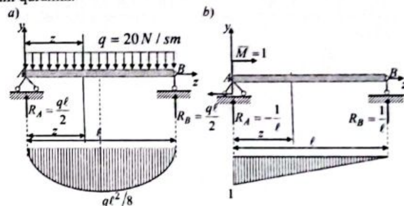
3.9-Tekis taqsimlangan yuk bilan yuklangan oddiy to'sin.
