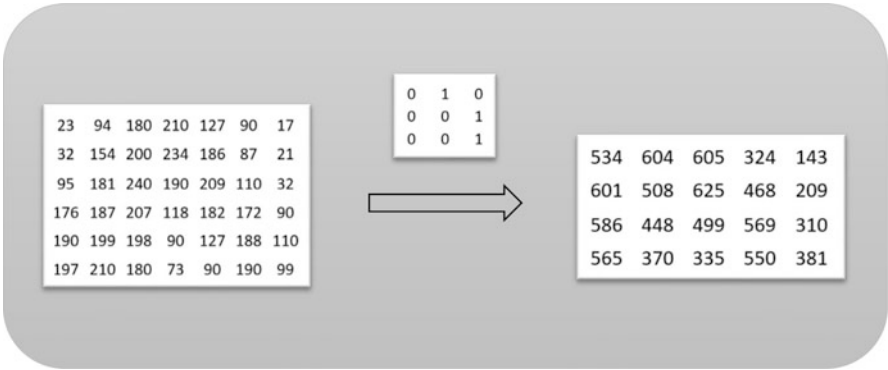
Fig. 16.4 Sliding the kernel along the pixel matrix on the left results in the (somewhat smaller) matrix on the right
