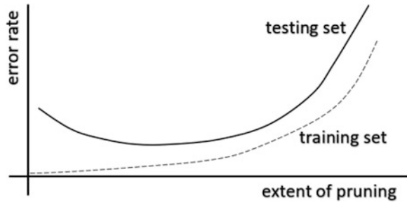
Fig. 5.3 With the growing extent of pruning (smaller trees), error rate on the testing set often drops, then starts growing again. Error rate on the training set usually increases monotonically
