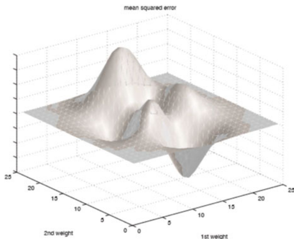
Fig. 6.3 For a given example, each set of weights results in a certain mean squared error. Training should reduce this error as quickly as possible, the steepest slope
