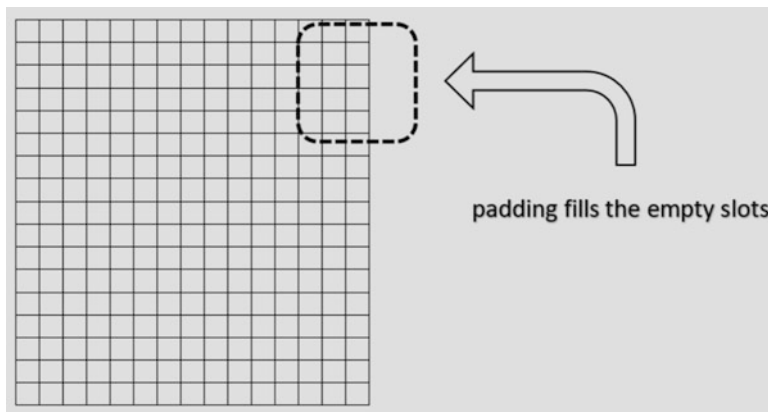
Fig. 16.6 Suppose the kernel's size is 5 \times 5 and the horizontal stride is s_x = 3 . At the end of the horizontal sliding, the kernel can reach beyond the end of the image. The “missing values” can be filled by padding
