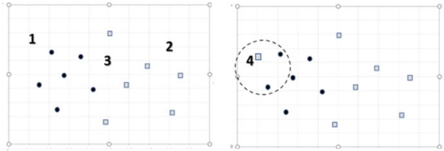
Fig. 3.1 Objects 1 and 2 find themselves deep in the “circles” and “squares” areas, respectively, and are thus easy to classify. Object 3, finding itself in the borderline region between the two classes, and its class is thus uncertain. In the class-noisy domain on the right, the 1-NN classifier will misclassify object 4, but the mistake is corrected if the 3-NN classifier is used
