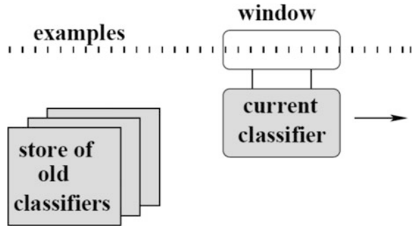
Fig. 11.3 A window passes over a stream of examples; “current classifier” is periodically updated to reflect changes in the underlying class. Occasionally, the system can retrieve some of the previous classifiers if the underlying context recurs
