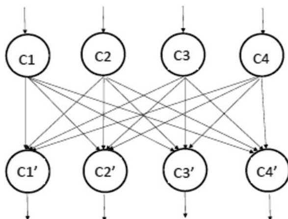
Fig. 14.2 Stacking . The upper-layer classifiers use as input the original attribute vector. For the lower-layer classifiers, this vector is extended by the class labels returned by the upper layer
