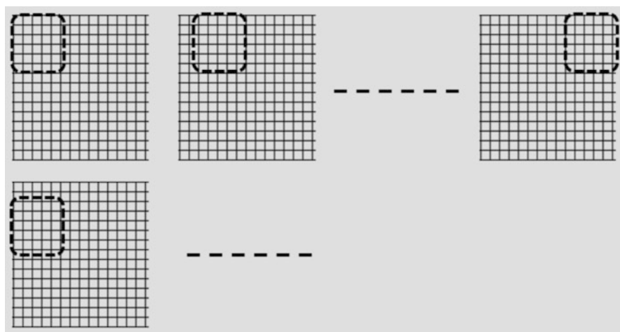
Fig. 16.5 In this picture the window is sliding with strides s_x = 2 and s_y = 2
