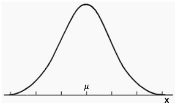
Fig. 2.3 For continuous-valued attributes, probability density function, p(x) , indicates the density of values in the vicinity of x . This graph shows the popular theoretical pdf : the Gaussian Bell Function
