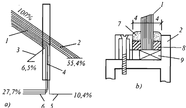
9.10-rasm. Shishaning issiqlikni yutish sxemasi:
