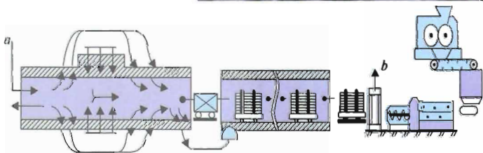
8.3-rasm. Sopol ashyolarini tunnel xumdonda kuydirish sxemasi:
