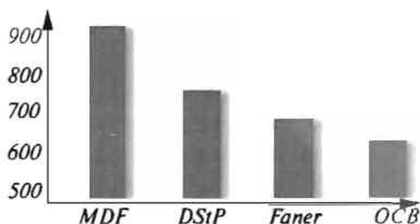
6.15-rasm. Zichligiga ko'ra taqqoslanganda MDF ning afzallik diagrammasi, \text{kg/m}^3 .
