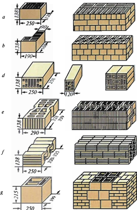
8.6-rasm. Yirik kovakli toshlar va ulardan devor terish:
