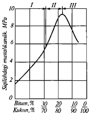
3.2-rasm. Mineral kukunining asfalt-beton mustahkamligiga ta'siri
