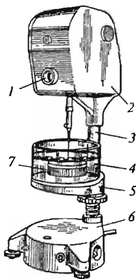
3.10-rasm. Penetrometr
