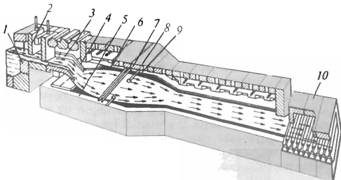
9.3-rasm. Shisha massani suyuq qalay eritmasida qoliplash:
