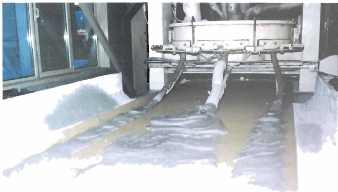
10.3-rasm. Gips qorishmasini karton tasмага yoyish.
