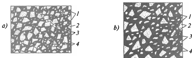
3.1-rasm. Asfalt-betonning tuzilishi:
