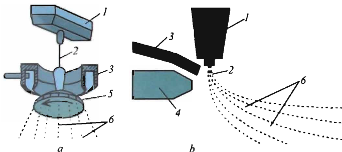
9.14-rasm. Shisha-tolasini (a) markazdan qochirma va (b) puflash usullarida tayyorlash sxemalari:
