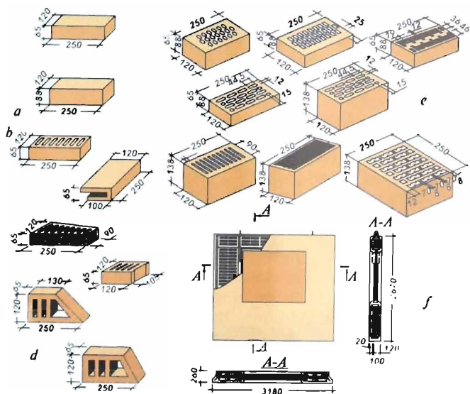
8.5-rasm. Devorbop sopol ashyolarning asosiy xillari:
