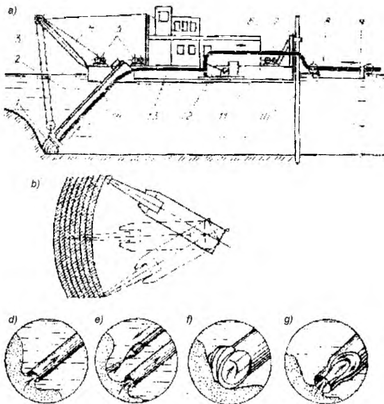
4.40-rasm. Zemsnaryadning ishlash sxemasi:
