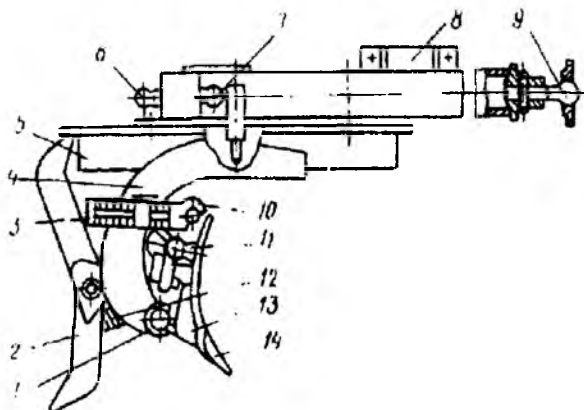
4.19-rasm. Avtogreyderning tortish ramasi:
