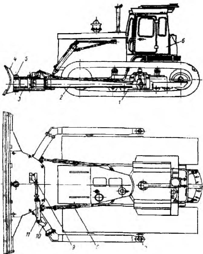
4.5-rasm. MK-21 kavaler tekislagichi:
