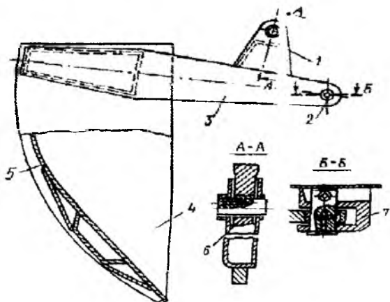
4.10-rasm. DZ-20V skreperining zaslonkasi:
