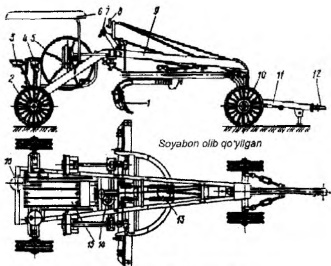
4.15-rasm. D-20 BMA greyderi:
