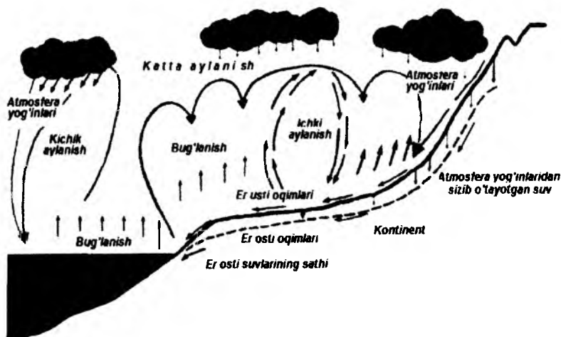
4-rasm. Tabiatda suvning aylanishi.
