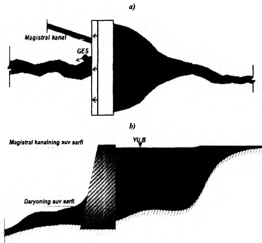
32-rasm. Kichik bosimli irrigatsion to'g'onga GESni o'rnatish sxemasi:
