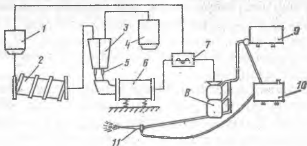
13.11 – rasm. Torkret yotqizish jihozining sxemasi:
