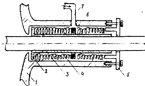
2.22-rasm. So'rish salnigi tuzilishi:
