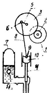
9.10 - rasm. Shtangali porshen nasos lebedkasi tasviri:
