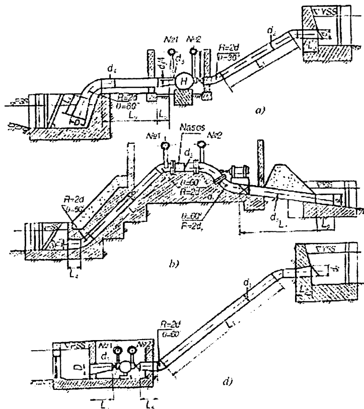
1.7-rasm. Nasos qurilmasining o'rnatilish shakllari
