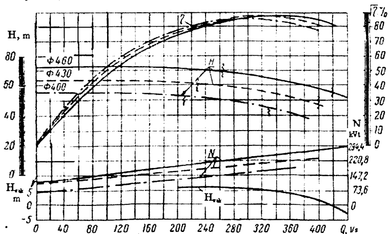
4.2- rasml. Markazdan qochma 12HD c nasosning xarakteristikasi( m=1450 ay/min).
