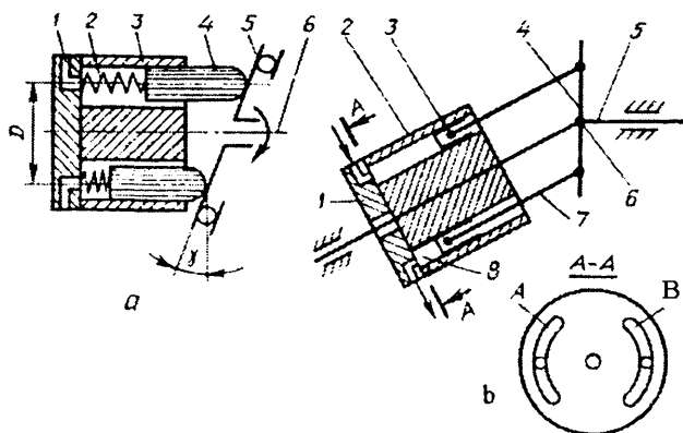
6.11-rasm. Aksial-porshenli nasos tasviri:
