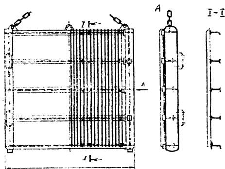
9.17- rasm. Yassi o'zakli panjara.
