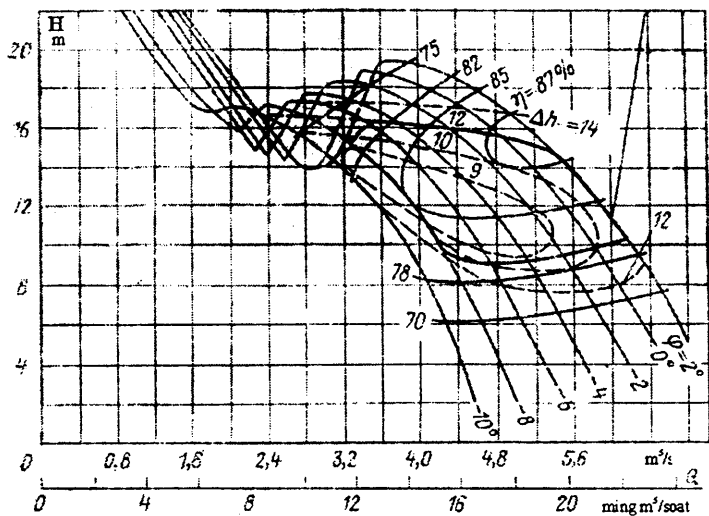
4.3-rasm. O'qiy OP2-110 nasosning universal xarakteristikasi ( n=485 ay/min).
