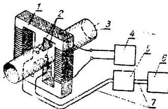
9. 25-rasm. Induksion sarf o'lhagichi:
