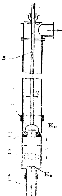
6.5- rasm. Vertikal shtangali porshen nasos tasviri:
