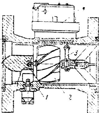
9.21- rasm Parrakli hajmiy hisoblagich: 1-qobiq; 2-parrak;, 3-uzatgich; 4-hisoblash mexanizmi.
