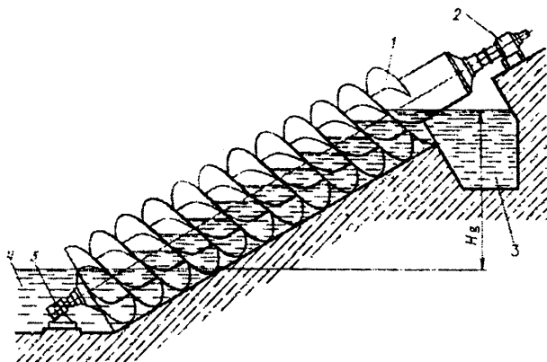
7.3-rasm. Shnekli nasosning o'rnatish tasviri:
