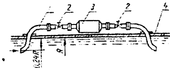
9.26 -rasm . Quvurlarga induksion sarf o'lchagichini parsial tasvirda o'rnatish:
