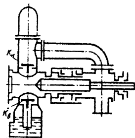
6.4-rasm. Differensial ishlovchi plunjerli nasos tasviri.
