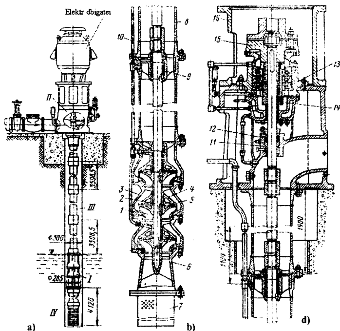
2.13-rasm. Transmission valli quduq nasosining tuzilishi:
