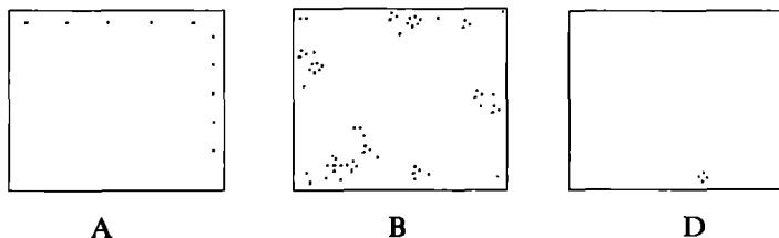
14-rasm. Populyatsiyada tur vakillarining uch xil taqsimlanishi
