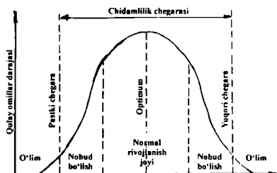
2-rasm. Ekologik omillarning ta'sir qilish natijalari (Radkevich, 1983)
