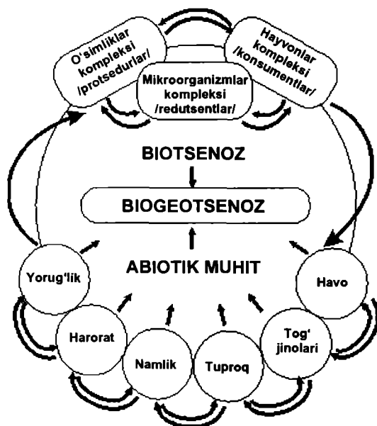
21-rasm. Biogeotsenoz ichidagi aloqalarning tuzilishi (Ponomareva, 1978)
