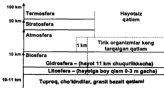
27-rasm. Biosferaning tuzilishi
