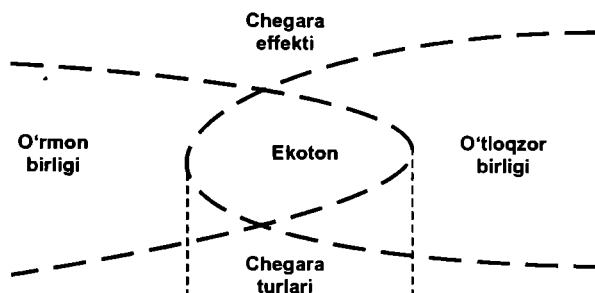
12-rasm. Ekotonning hosil bo'lishi (original)
