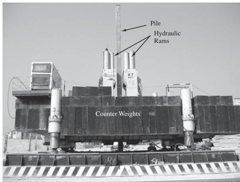
Figure 12.51 Installation of precast concrete piles with a pile jacking rig. A crane picks up a pile and feeds it into the center of the jacking rig where a set of hydraulic clamps grab the pile and then push it into the ground (courtesy of Limin Zhang, Hong Kong University of Science and Technology).
