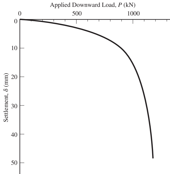
Figure 14.14 Static load test results for Problems 14.3 and 14.4.
