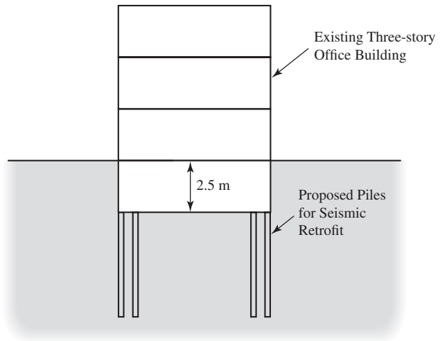
Figure 5.12 As part of a seismic retrofit project, a design engineer has called for installing 450 mm diameter, 9 m long prestressed concrete pile foundation to be installed beneath the basement of an existing building. This pile foundation design is unbuildable because the required pile-driving equipment would not fit in the basement, and because there is not enough room to set the pile upright.
