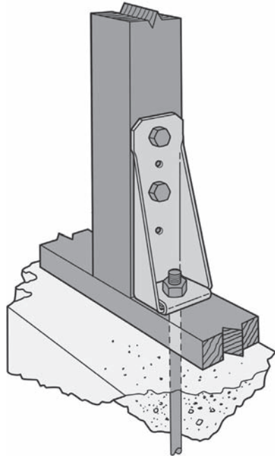
Figure 10.28 Use of steel holdown bracket to connect a wood-frame wall with large uplift force to a footing.
