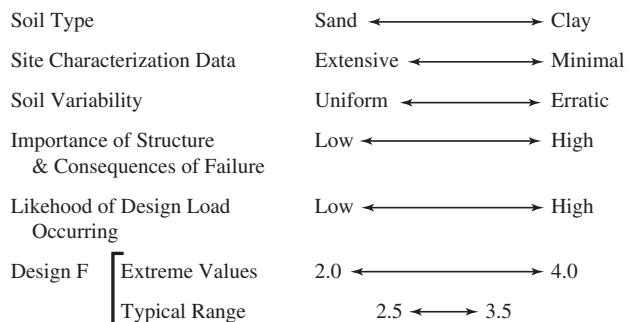
Figure 7.12 Factors affecting the design factor of safety, and typical values of F .
