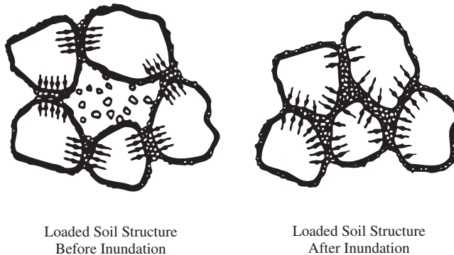
Figure 28.1 Microscopic view of a collapsible soil. In their natural state, these soils have a honeycomb structure that is held together by water soluble bonds. However, if the soil becomes wet, these bonds soften and the soil consolidates (based on from Houston et al., 1988; used with permission of ASCE).
