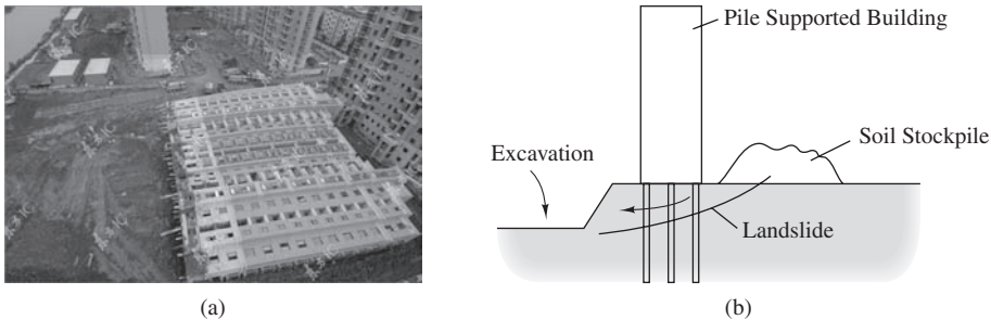
Figure 23.6 On June 27, 2009 a 13-story supported Shanghai apartment building collapsed while under construction as seen in (a). The collapse was due not a foundation failure per se, but to a landslide caused by creating both an excavation on one side of the building and a soil stockpile on the other side as shown in (b).
