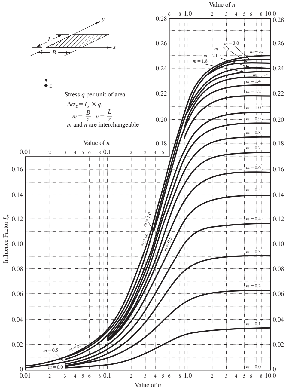
Figure 3.8 Influence factors for induced vertical stress beneath the corner of a rectangular loaded area (U.S. Navy, 1982).
