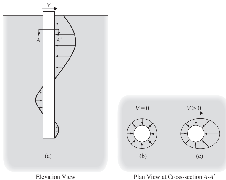
Figure 13.5 Load transfer in a laterally loaded pile. (a) Shows the vertical distribution of the net lateral force applied to the pile by the surrounding soil. (b) and (c) Show the distribution of lateral stress around the pile at a given cross section for different values of shear force at the top of the pile, V . (b) Shows a uniform distribution of lateral stress which occurs when the shear force is zero. As the shear force is increased, the lateral stress increases in the direction of pile displacement and decreases on the opposite side of the pile as shown in (c).
