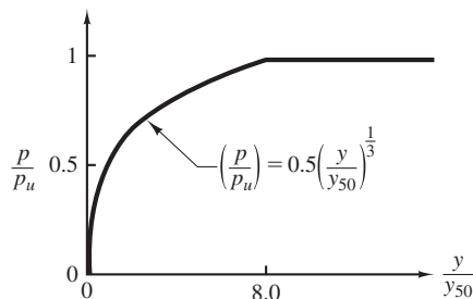
Figure 22.14 Matlock's p - y curve for static loading of an isolated pile in soft cohesive soil.
