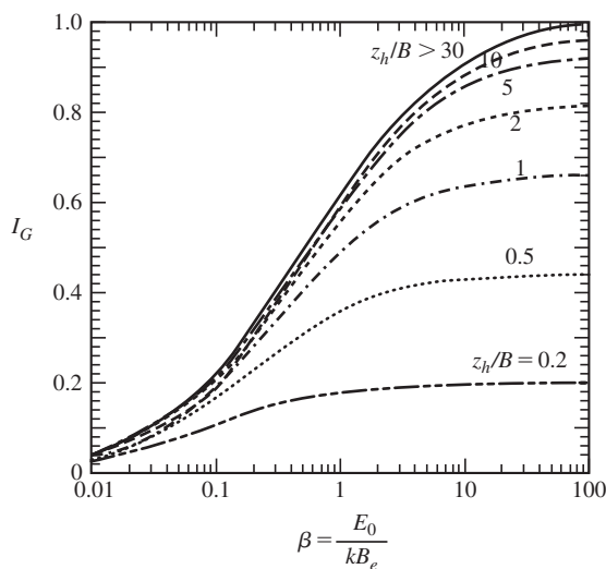
Figure 8.4 Chart to determine I_G in the Mayne and Poulos (1999) method for computing settlement.
