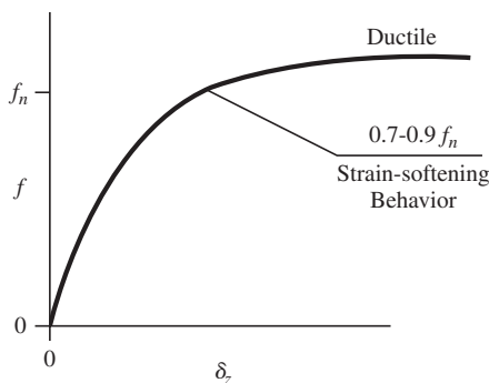
Figure 20.2 Ductile and strain-softening behavior.
