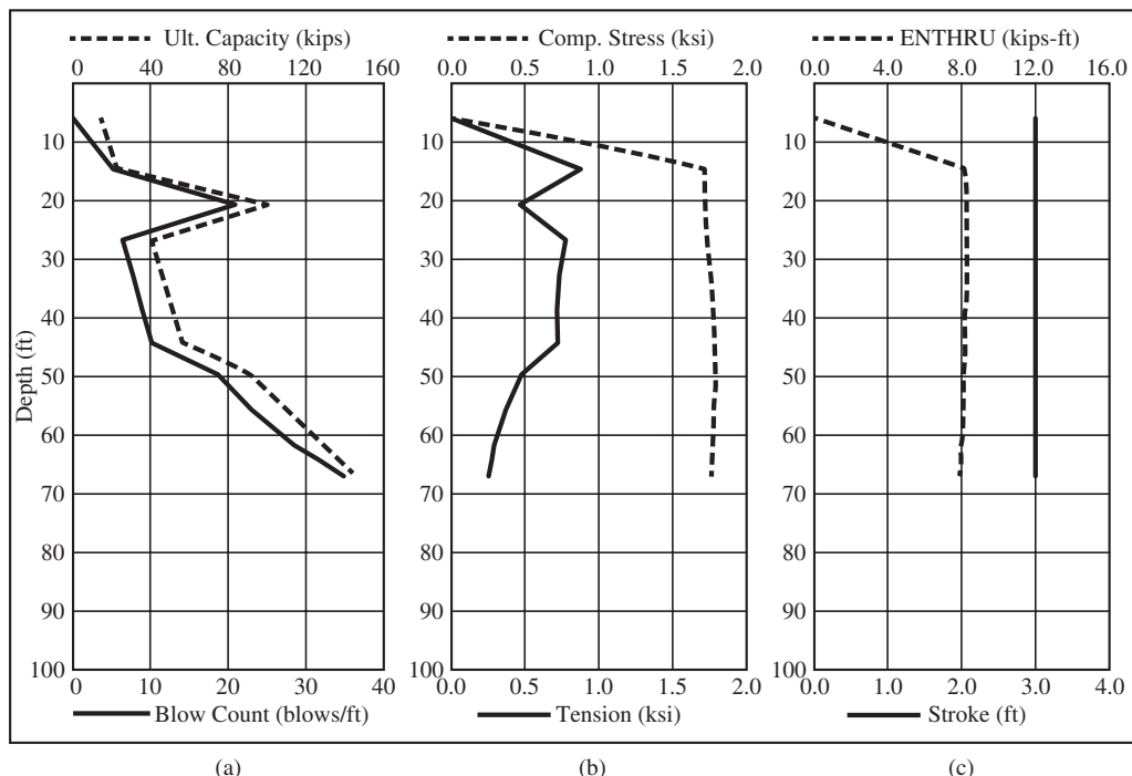
Figure 19.7 Results of a typical driveability analysis: (a) shows static pile capacity and blow count as a function of depth; (b) shows maximum compressive and tensile stress in the pile as a function of depth; (c) shows the hammer stroke (for a diesel hammer) as a function of depth (data generated using GRLWEAP).
