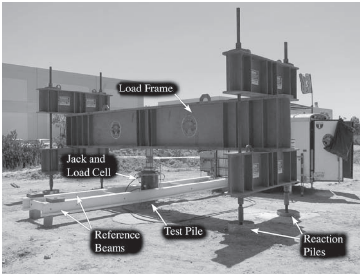
Figure 14.2 A static load test using a beam and reaction piles to develop the test load.
