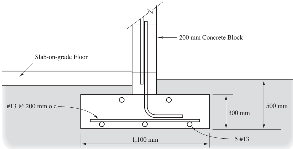
Figure 10.14 Final design for Example 10.2.
