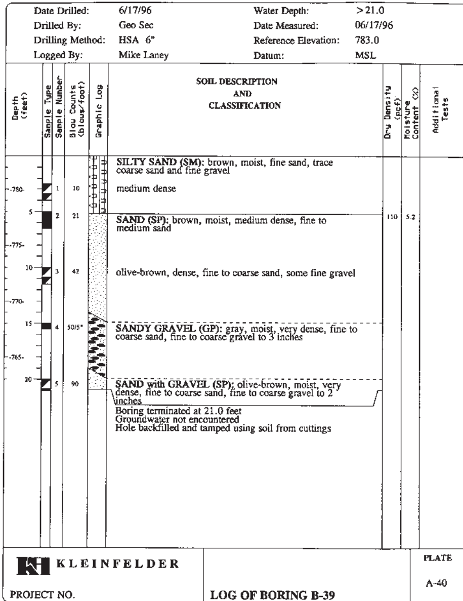
Figure 4.4 A boring log. Samples 2 and 4 were obtained using a heavy-wall sampler, and the corresponding blowcounts are the number of hammer blows required to drive the sampler. Samples 1, 3, and 5 are standard penetration tests, and the corresponding blowcounts are the N_{60} values, as discussed later in this chapter. If the groundwater table had been encountered, it would have been shown on the log (Courtesy of Kleinfelder, Inc.).
