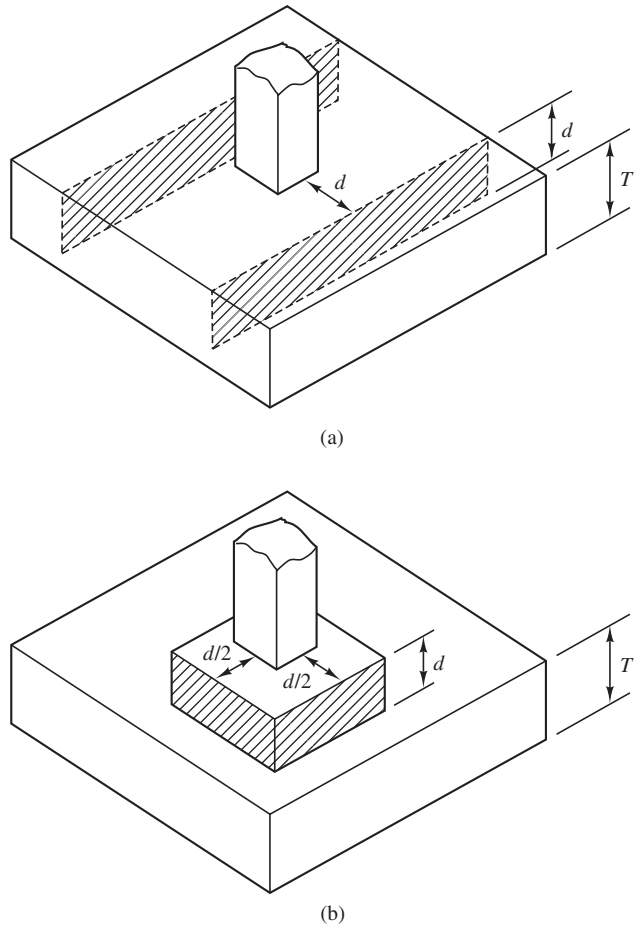
Figure 10.5 The two modes of shear failure: (a) one-way shear; and (b) two-way shear.
