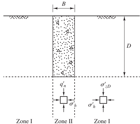
Figure 25.16 Stress conditions for lower bound solution for toe bearing of a rock socket (after Kulhawy and Carter, 1992).
