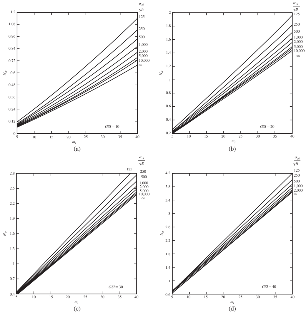
Figure 25.12 Bearing capacity factor, N_g , for a circular footing, based on finite element analyses: (a) GSI = 10, (b) GSI = 20, (c) GSI = 30, (d) GSI = 40 (Clausen, 2013).
