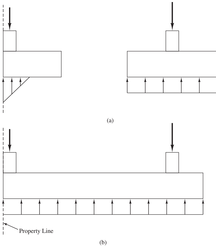
Figure 9.6 Combined footing to eliminate eccentric loading: (a) shows two adjacent footings; the footing on the left is eccentrically loaded because the property line prevents locating the column in the center of the footing. (b) By combining the two footings, it is possible to create a uniform bearing stress across the combined footing.
