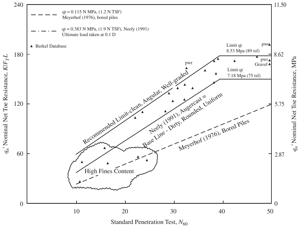
Figure 17.7 Experimental q'_t values derived from load tests on DD piles and SPT results (NeSmith, 2002).
