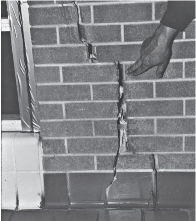
Figure 27.1 Heaving of expansive soils caused this brick wall to crack. The $490,000 spent to repair this and other walls, ceilings, doors, and windows represented nearly one-third of the original cost of the six-year-old building (photo courtesy of the Colorado Geological Survey).
