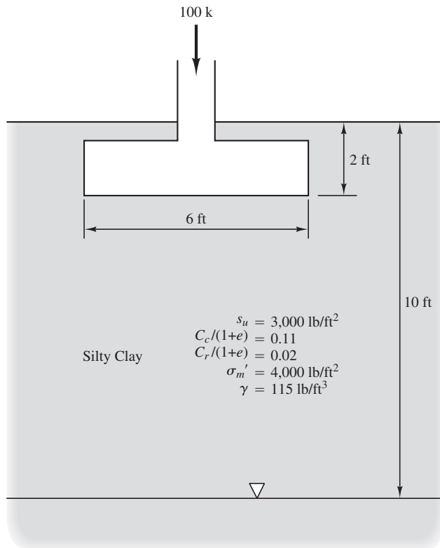
Figure 8.10 Proposed spread footing for Example 8.6.
