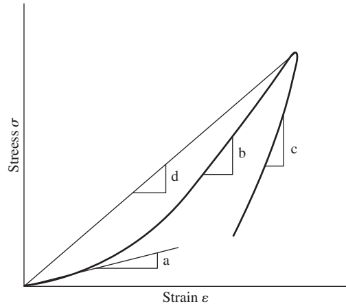
Figure 25.6 Definitions of different moduli used to describe rock mass behavior: (a) initial tangent modulus, (b) elastic tangent modulus, (c) recovery (unload) modulus, and (d) secant modulus (after Hoek and Diederichs, 2006).
