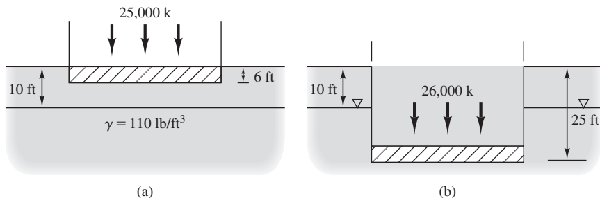
Figure 11.4 Mat for Example 11.1.
