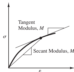
Figure 3.10 Stress-strain curve for one-dimensional compression showing the secant formulation versus the tangent formulation of constrained modulus, M , for a given point on the stress-strain curve.
