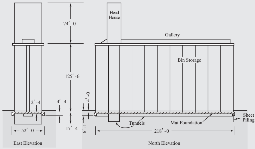
Figure 7.13 Elevation views of the elevator (Based on Nordlund and Deere, 1970; reprinted by permission of ASCE).
