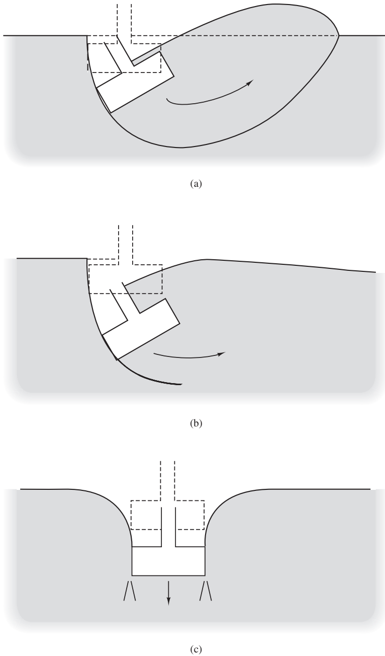
Figure 7.1 Modes of bearing capacity failure: (a) general shear failure; (b) local shear failure; and (c) punching shear failure.
