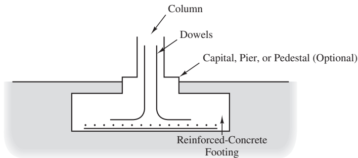
Figure 6.6 Reinforced-concrete spread footing.
