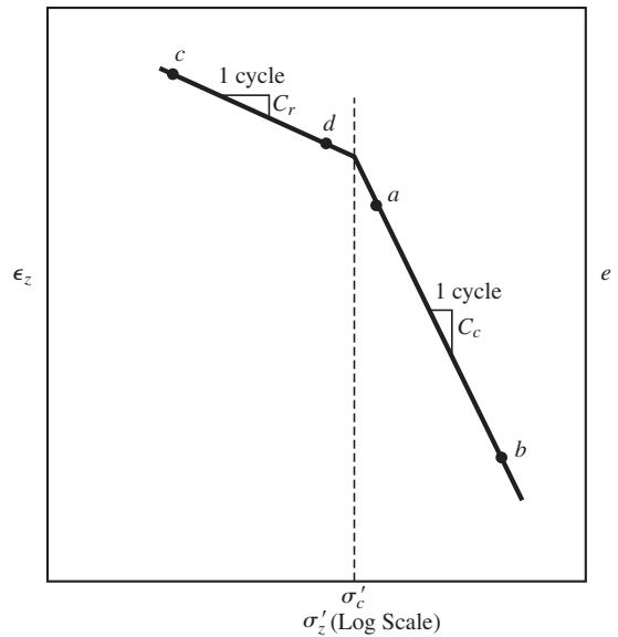
Figure 4.11 Illustration of an idealized bilinear e -log- p curve. The slopes of the two parts of the curve on a semilogarithmic e versus \sigma'_z plot are C_c and C_r . The break in slope occurs at the preconsolidation stress, \sigma'_c .
