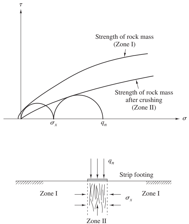
Figure 25.9 Method for analyzing bearing capacity of footings on rock (after Goodman, 1989).
