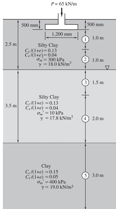
Figure 8.11 Proposed footing for Example 8.2.
