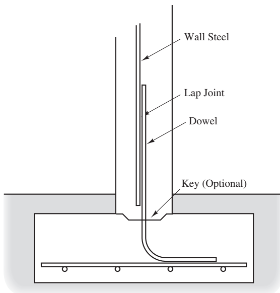
Figure 10.17 Use of dowels to connect a concrete or masonry column to its footing.
