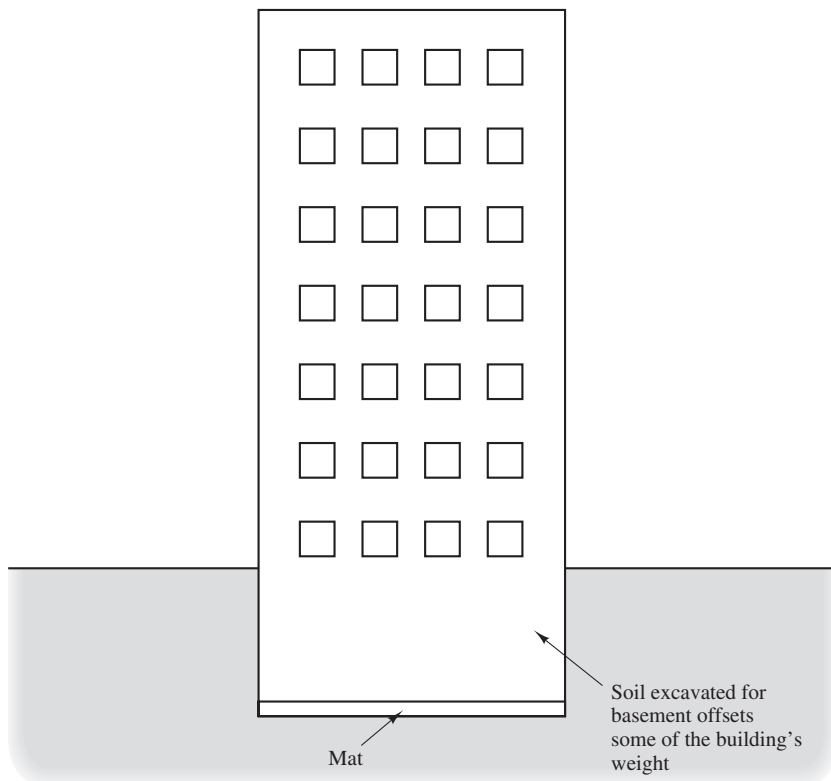
Figure 11.3 A compensated mat foundation.
