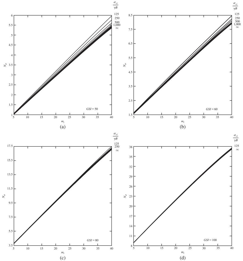
Figure 25.13 Bearing capacity factor, N_\sigma , for a circular footing, based on finite element analyses: (a) GSI = 50 , (b) GSI = 60 , (c) GSI = 80 , (d) GSI = 100 (Clausen, 2013).
