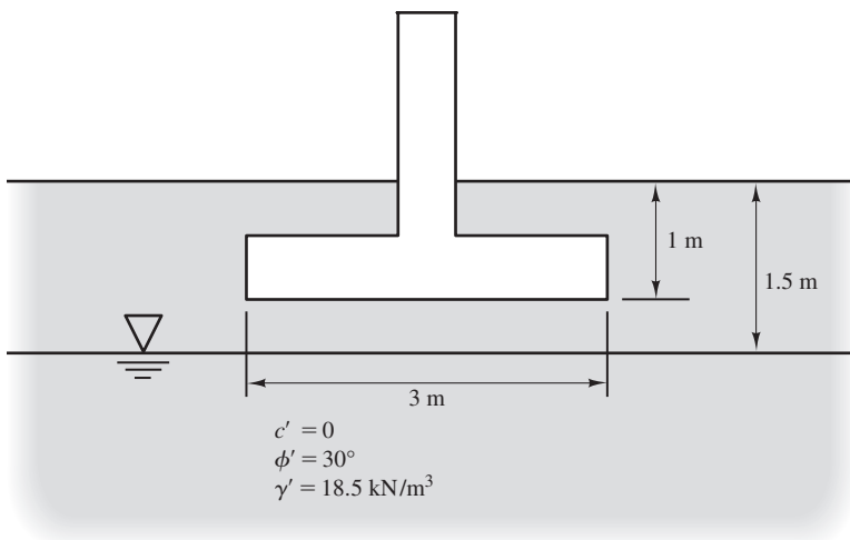
Figure 7.11 Proposed footing for Example 7.3.
