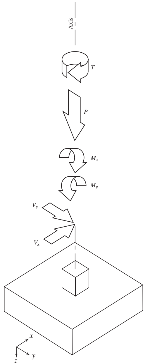
Figure 5.2 Types of structural loads acting on a foundation.
