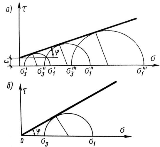
2.13-rasm. Stabilometrdagi sinov-lar bo'yicha gruntning mustahkamlik ko'rsatkichlarini aniqlash: a – bog'lanishli grunt; b – sochiluvchan grunt
