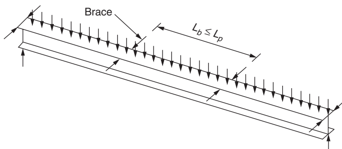
FIGURE 4.2 Beam bracing.
