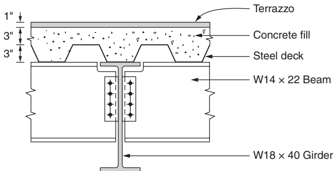
FIGURE 2.6 Girder detail.
