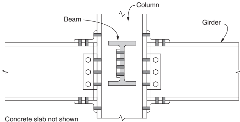
FIGURE 1.8 Column detail.
