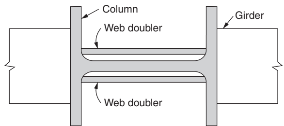
FIGURE 6.22 Alternative web doubler plate detail.
