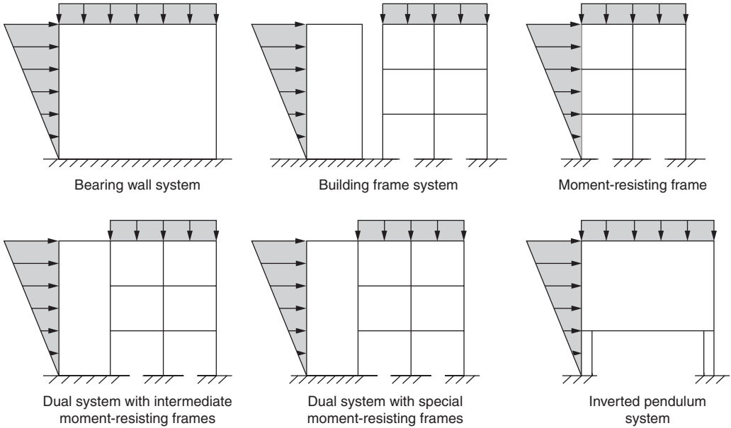
FIGURE 2.42 Structural systems.
