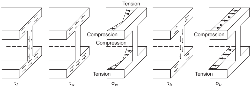
FIGURE 5.12 Torsion effects in a W-shape.
