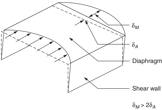
FIGURE 2.46 Flexible diaphragm.
