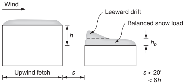
FIGURE 2.16 Drift formed on adjacent low structure.
