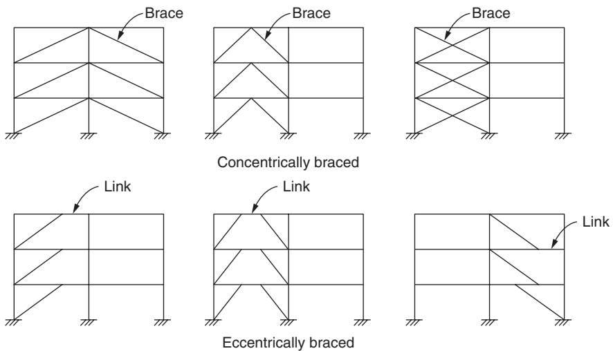
FIGURE 1.10 Braced frames.
