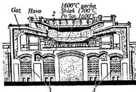
10.9-rasm. Marten pechi sxemasi 1. tag; 2. gumbaz; 3 regenerators.
