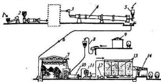
5.10-rasm. Portland sement ishlab chiqarish sxemasi.
