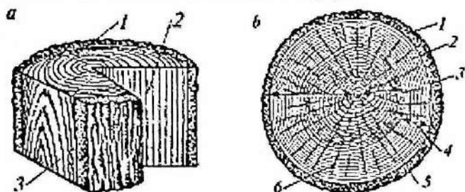
13.1-rasm. Yog'och tanasining tuzilishi.
