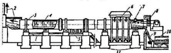
5.9-rasm. Aylanma xumdon.
