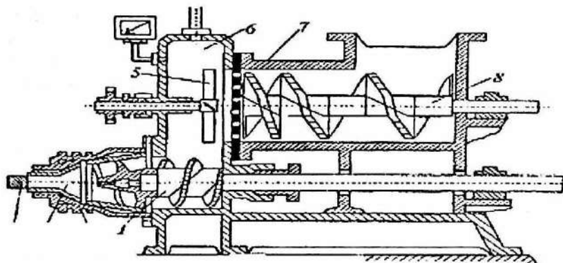
3.2-rasm. Tasmali hamda vakuumli press.
