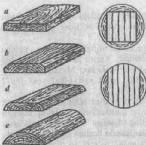
2.15-rasm. Yog'och taxtalar: a -har tomoni tilingan toza taxta; b -yarim tilingan taxta; d -qirrasi tilinmagan taxta; e -pushtaxta.
