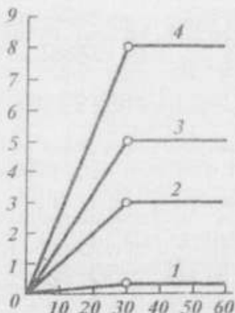
2.10-rasm. Namlikni yog'ochning shishishiga ta'siri: 1-tolalari bo'ylab; 2-radial yo'nalishi; 3-tangential yo'nalishi; 4-hajmiy shishish.
