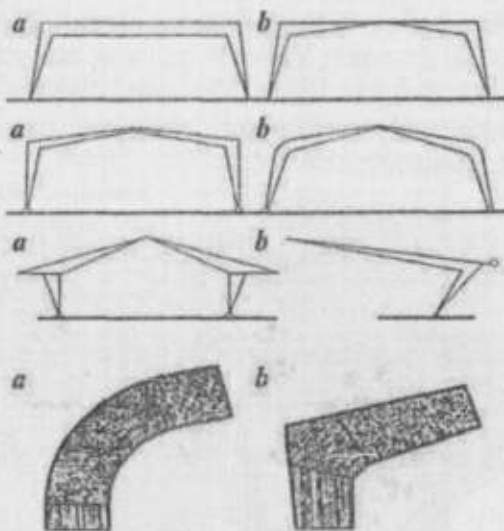
2.2-rasm. Yelimlangan yog'och rom turiari.
