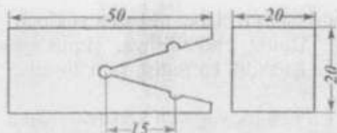
2.12-rasm. Yog'ochni yoriluvchanlikka sinash uchun tayyorlangan namuna.
