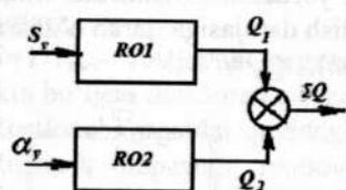
6.4 – rasm. Murakkab rostlash organning funksional sxemasi.
