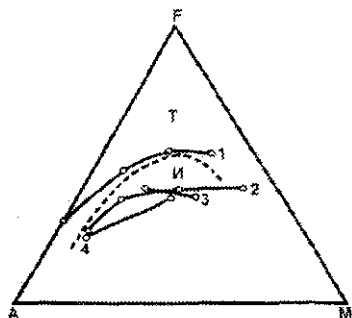
4.4-rasm. AFM diagrammasida har xil kimyoviy seriyalar o'rni (Irwin, Baragar, 1971).
