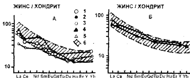
4.28-rasm. Nodir elementlarning Killipek va Korall orollarida tarqalishi (xondritga nisbatan).
