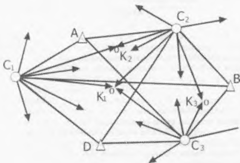
2.8-rasm. Ozod bekatlar taximetriyasini bajarish sxemasi
