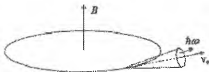
3.2-rasm. Sinxrotron nurlanishning yo'nalishi.
