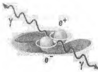
4.5-rasm Gamma-kvant hosil bo'lishi
