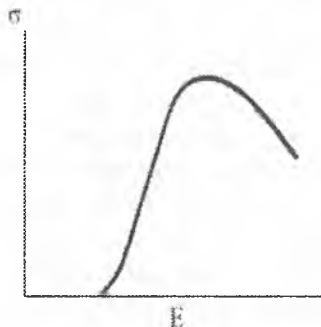
5.18-rasm. Reaksiya kesimining zaryadlangan zarra energiyasiga bog'lanishi
