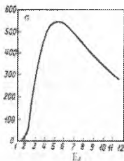
5.17-rasm. ^{23}\text{Na}(d,p)^{24}\text{Na} reaksiyaning uyg'onish funksiyasi
