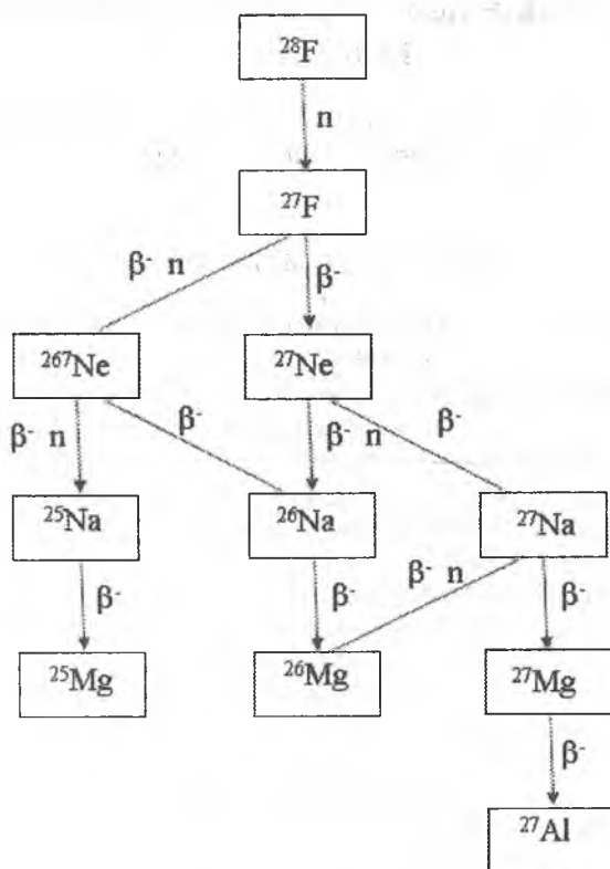
1.27-rasm. ^{28}\text{F} izotopining parchalanishi.
