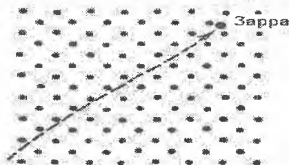
3.5-rasm. Zaryadlangan zarralarning kristallarda kanallashuvi
