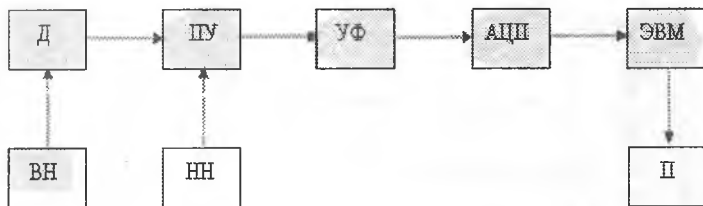
5.25-rasm. O'lchash kompleksining blok-sxemasi: D – Ge-detektor; PU – oldingi kuchaytirgich; UF – kuchaytirgi-impulslarni shakillatgich (formirovatel); VN – yuqori kuchlanish manbai; NN – past kuchlanish manbai; ATSP – analogoi-raqamli aylantirgich; EVM – Pentium-4; P – printer HP Laser Jet 1000
