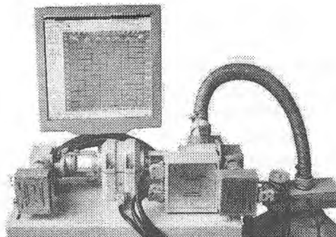
1.15-rasm. MS-1104Em turdagi Myossbauer spektrometri
