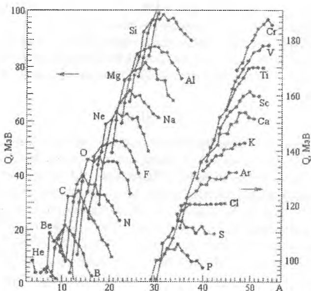
1.18-rasm. ^{208}\text{Pb} og'ir fragmenti hosil bo'lishiga olib keluvchi turli parchalanishlar uchun klaster Q parchalanish energiyasining chiqayotgan klaster massa soniga bog'lanishi.
