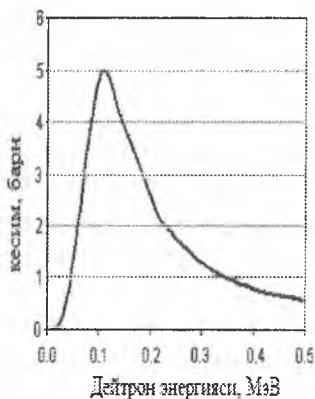
5.6-rasm. t(d,n)^4\text{He} reaksiya uchun uyg'onish funksiyasi
