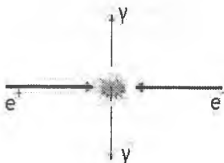
4.4-rasm Gamma-kvant hosil bo'lishi
