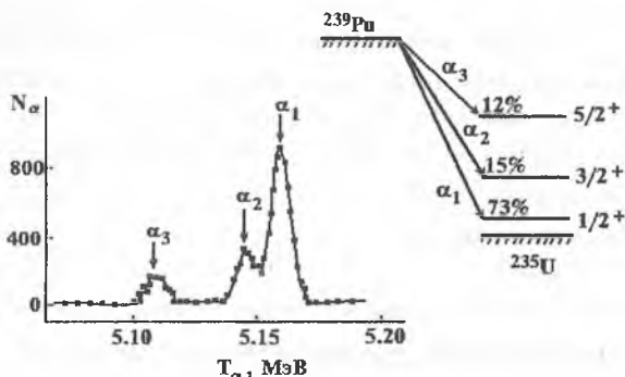
1.3–rasm. Plutoniy ^{239}\text{Pu} yadrosining \alpha -parchalanish sxemasi.
