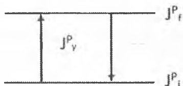
1.8-rasm. Yadroda radiatsion o'tishlar.
