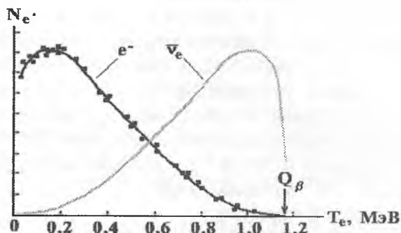
1.4-rasm. ^{210}_{83}\text{Bi} \rightarrow ^{210}_{84}\text{Po} + e^- + \bar{\nu}_e parchalanishda hosil bo'ladigan elektron va neytrinning energetik spektrlari.
