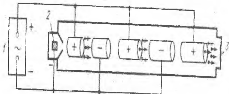
5.13-rasm. Chiziqli rezonans tezlatgich: 1-YuCh-generator; 2-ionlar manbai; 3-nishon
