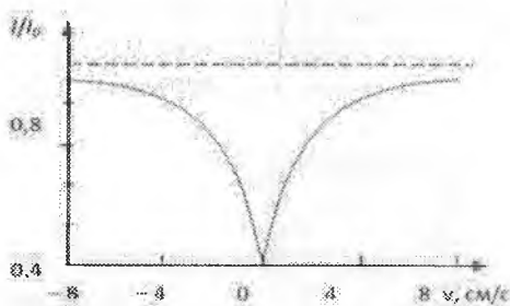
1.14-rasm. Myossbauer tajribasida olingan yutilish egri chiziq
