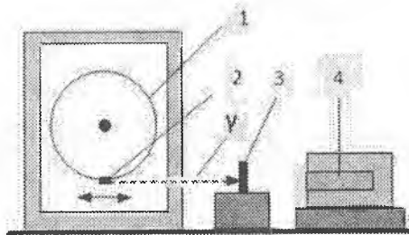
1.13-rasm. Myossbauer tajribasi
