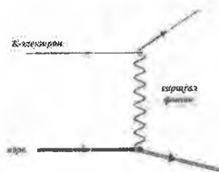
1.10-rasm. Ichki konversiya jarayonining Feynman diagrammasi
