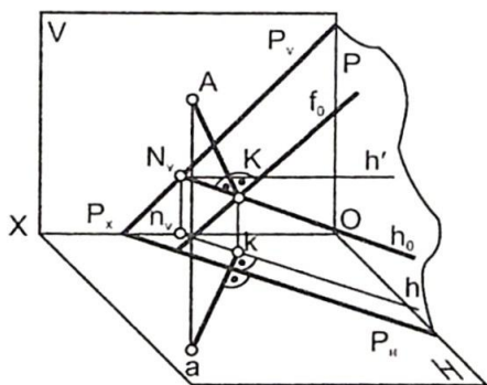
4.13-chizma
