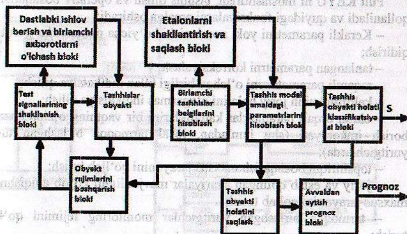
15.5-rasm. Tashhislash jarayonining namunaviy tuzilish sxemasi
