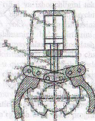
14.9-rasm. Pnevmo yuritmalari ushlagich qurilma
