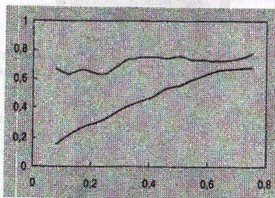
17.5-rasm. Quvvat koeffitsienti ( 1 - \cos \varphi ; 2 - \cos \varphi_{opt} ) qiymatlarini yuklanish bo'yicha o'zgarishi
