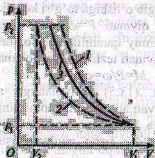
13.3-rasm . Gazning siqilishining indikatorli diagrammasi
