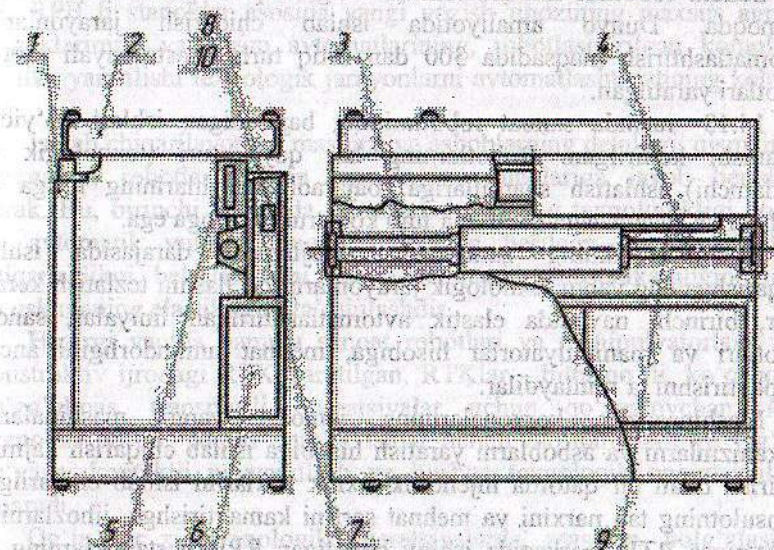
14.12-rasm. Yuklash qurilmasi
