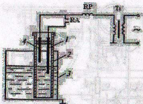
13.11-rasm . Elektrodli rele tuzilishi
