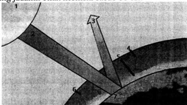
1.2-rasm Issiqxona effekti
