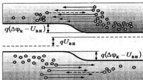
3.1-rasm. p-n o'tishning sohalar diagrammasi.
