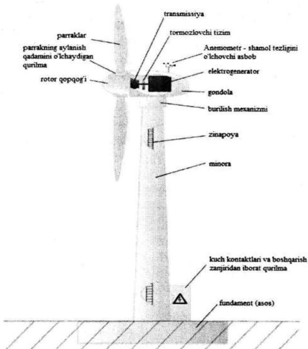
5.9-rasm. Shamol generator qurilmasi [22].
