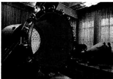
4.9-rasm. Atom bombasining hozirgi vaqtdagi ko'rinishi.
