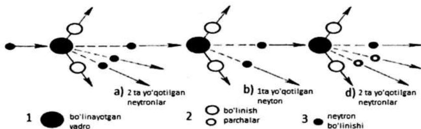
4.3-rasm. Atom parchalanishining zanjir reaksiyasi.
