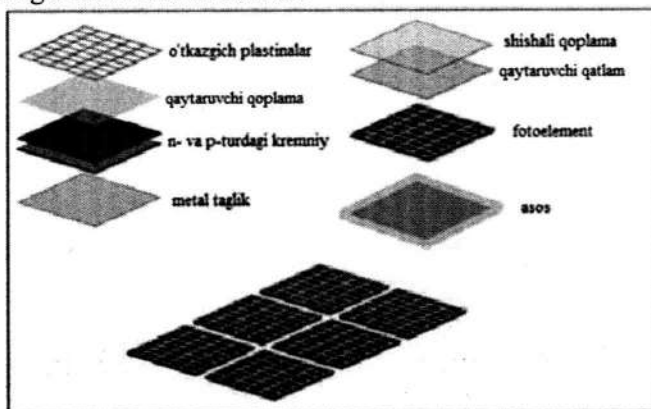
3.10-rasm. Quyosh panelining tuzilishi.
