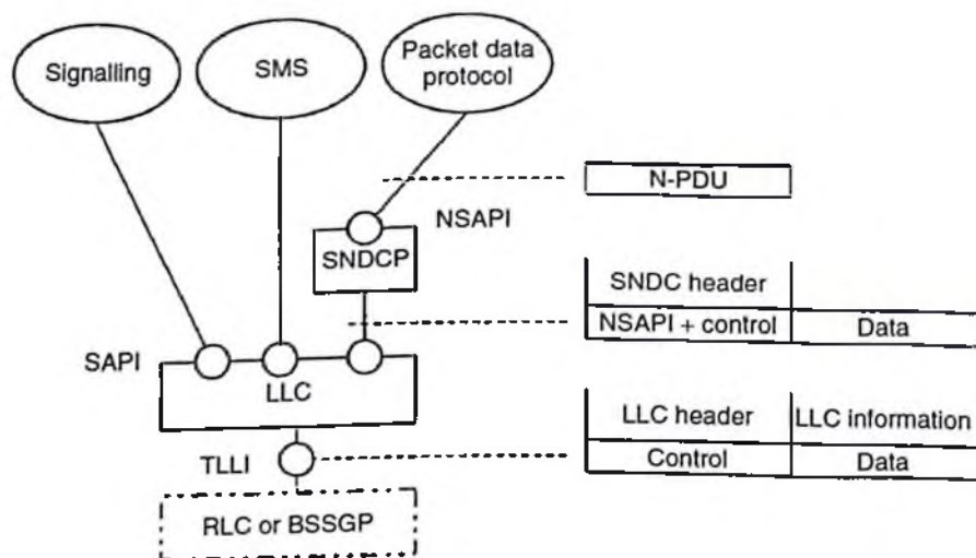
2.1-rasm. Tizimli protokollarni multipleksirlash.
