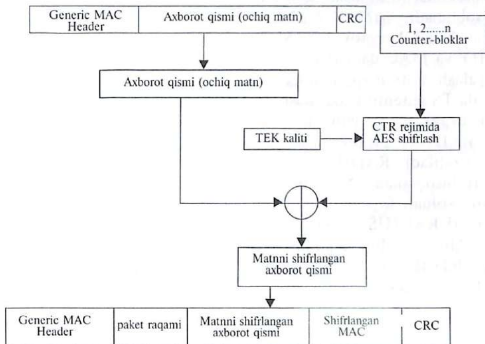
36.5-rasm. Xabarni axborot qismini shifrlash.
