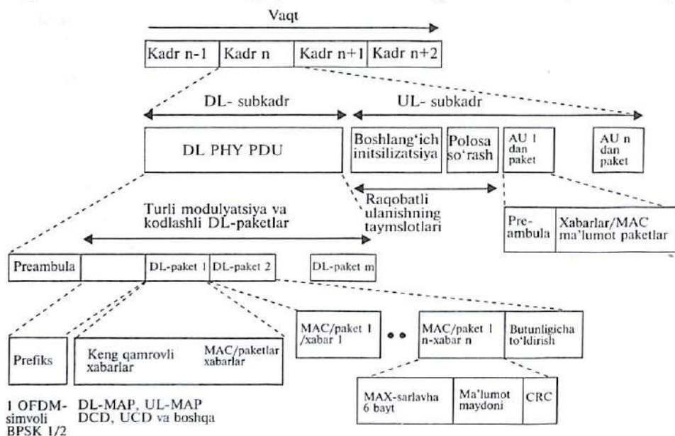
29.4-rasm. TDDli OFDM kadrning tuzilmasi.
