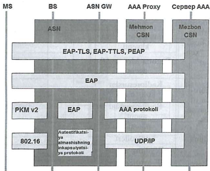
36.8-rasm. WiMAX tizimida AAA uchun protokollar steki.
