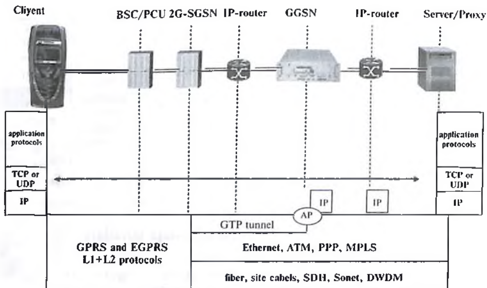
3.5-rasm. IP paketidan GPRS protokoliga o'tish.
