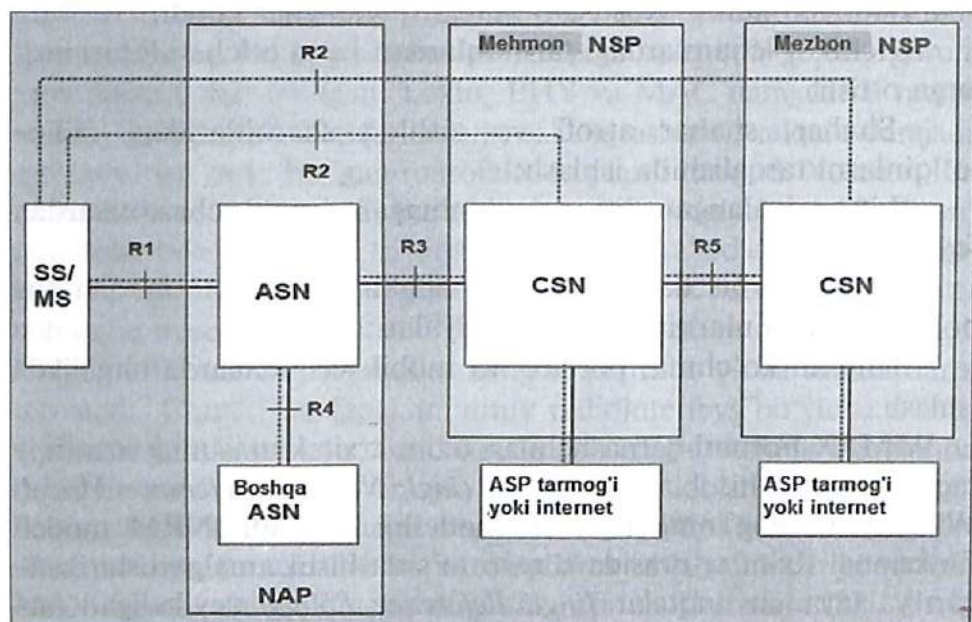
28.1-rasm. WiMAX tarmog'ining tayanch modeli (NRM).
