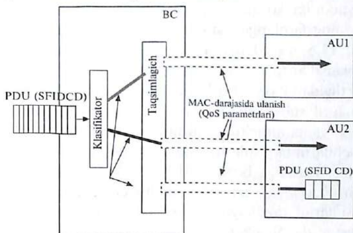
29.5-rasm. IEEE standartida QoSni qo‘llab-quvvatlash.
