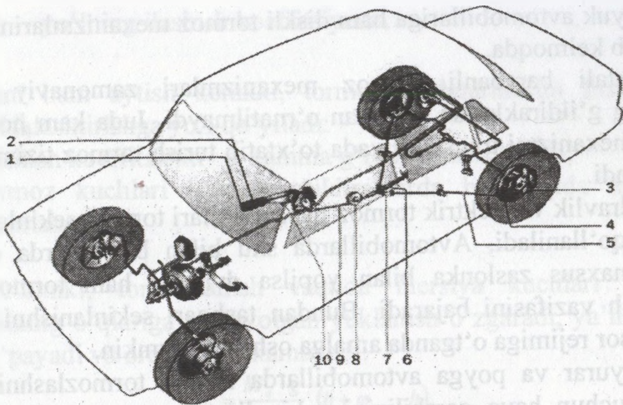
12.2-rasm. To'xtatib turish tormoz tizimi
