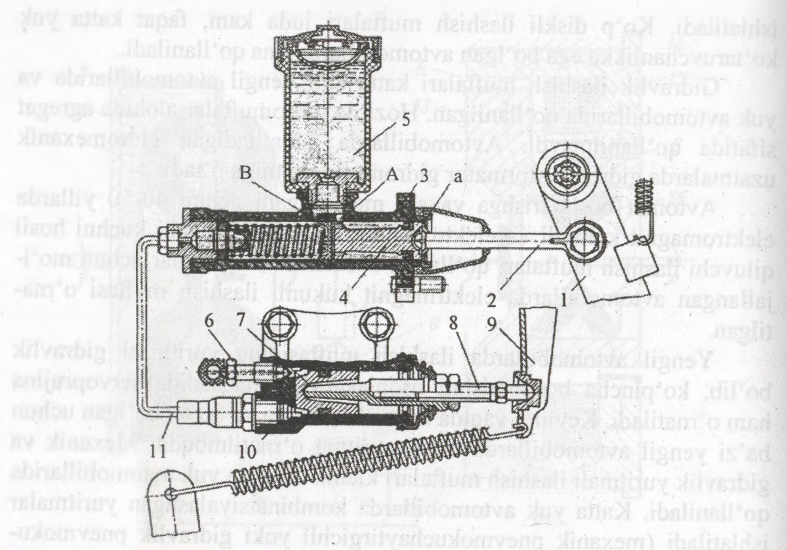
5.4-rasm. Ilashish muftasining gidravlik yuritmasi
