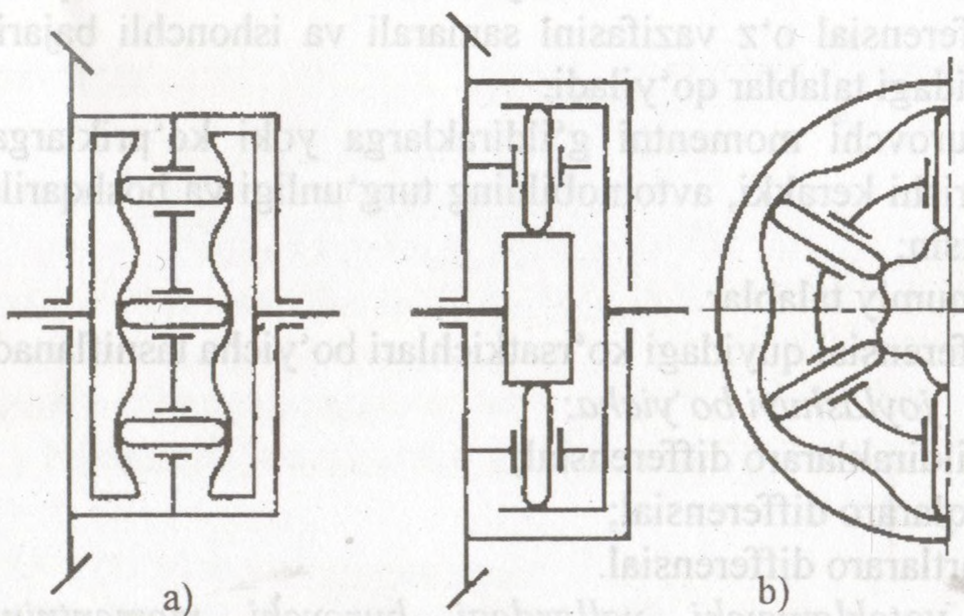
9.2-rasm. Mushtchali differensial sxemalari:
