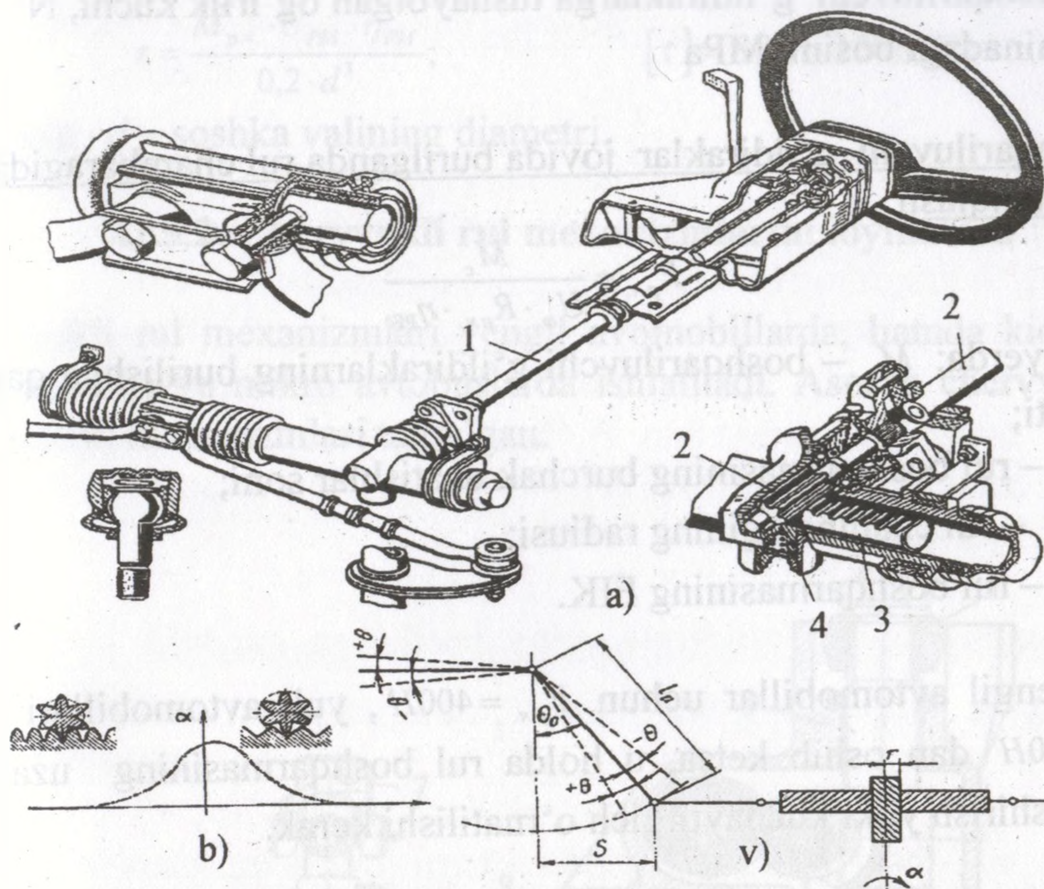
11.2-rasm. Shesternya-reykali rul mexanizmi:
