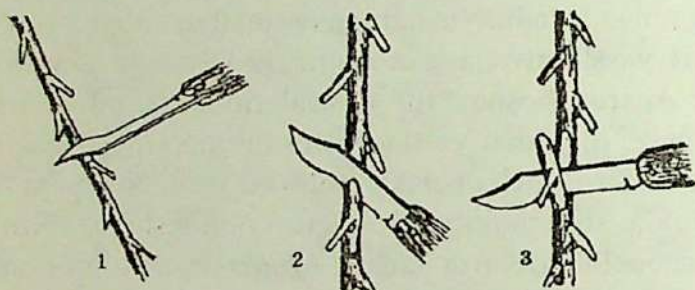
29- rasm. T-shakldagi payvand uchun payvandustni tayyorlash: 1—po'stloqni ko'ndalang kesish; 2, 3—payvandlanadigan kurtakni ajratish.
