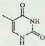
Timin
