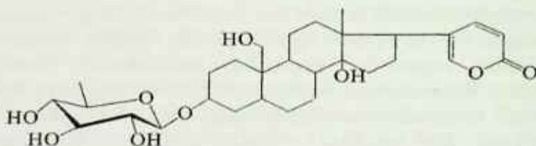
Bufodienolid gellebrigenol
