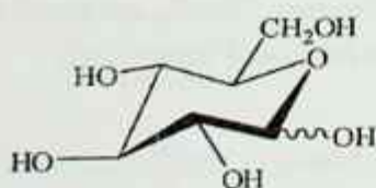
\alpha\text{-D-glukoza}
