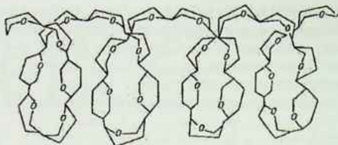
2-rasm. Amiloza molekulasining tuzilishi
