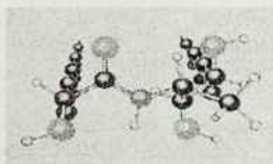
9-rasm. Seramid molekulasining konformatsiyasi
