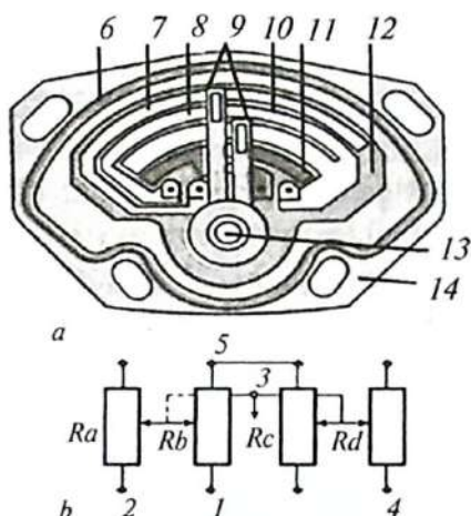
6.6-rasm. Drossel to'siqchasi holati datchigi:
