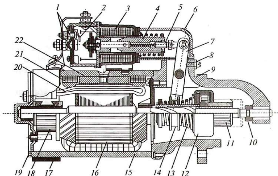
2.5-rasm. CT130-A3 belgili starter:
