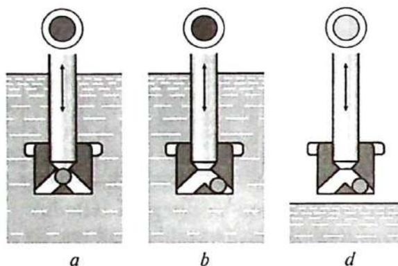
1.7-rasm. Akkumulatorning zaryadlanganlik darajasini ko'rsatuvchi indikator:
