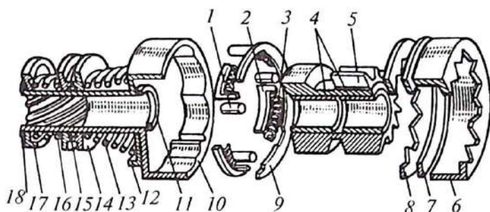
2.11-rasm. Plunjersiz rolikli erkin yurish muftasi:
