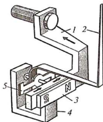
4.10-rasm. Elektromagnitli tizimdagi ampermetr.
