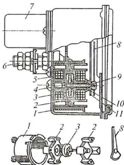
4.2-rasm. Logometrik ko'rsatkich.
