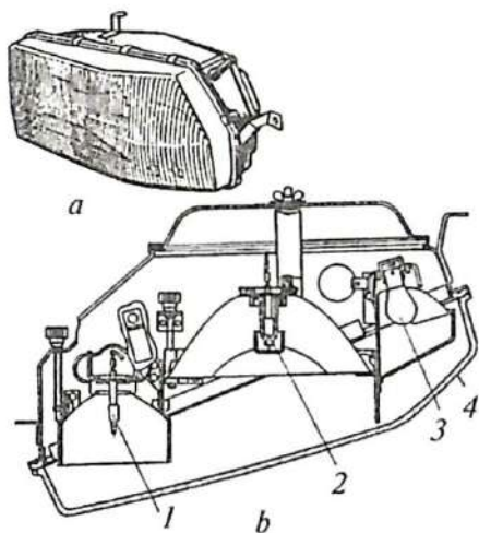
5.6-rasm. Blok-fara:
