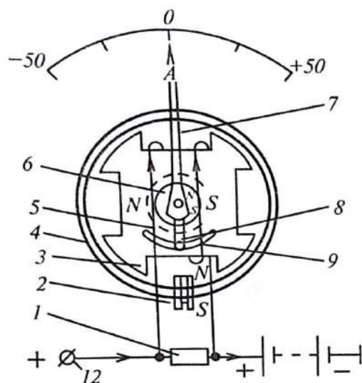
4.11-rasm. Magnitoelektr tizimidagi ampermetr.
