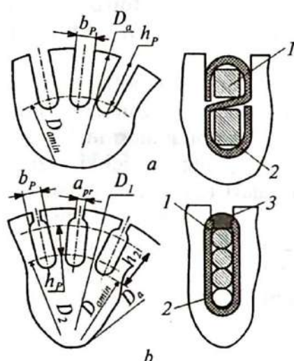
2.6-rasm. Starter yakori ariqchalarining chizmasi:
