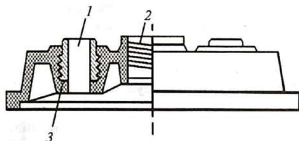
1.2-rasm. Akkumulator qopqog'i.
