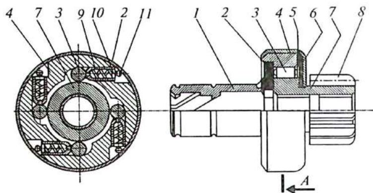
2.10-rasm. Plunjer-rolikli erkin yurish muftasi.
