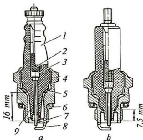
3.26-rasm. O't oldirish shaming tuzilishi:
