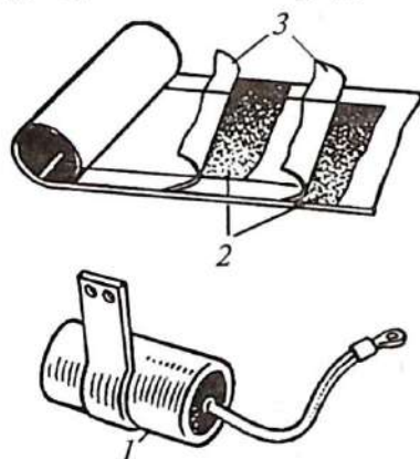
3.12-rasm. Kondensator.
