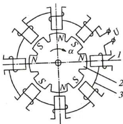
3.15-rasm. Magnitoelektr datchik chizmasi: 1—magnit; 2—stator; 3—chulg'am.
