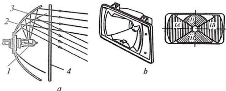
5.7-rasm. Gomofokal faraning optik tizimining chizmasi:
