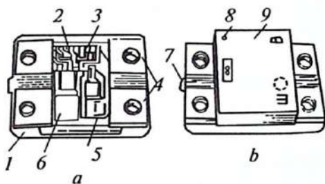
1.33-rasm. Я112A integral rostlagichi:
