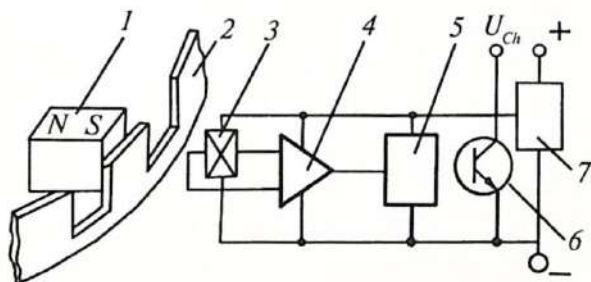
3.18-rasm. Xoll datchigi.
