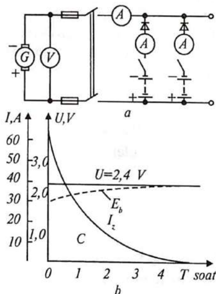
1.11-rasm. Akkumulatorlar batareyasining kuchlanishi o'zgarmas bo'lganda zaryadlash:
