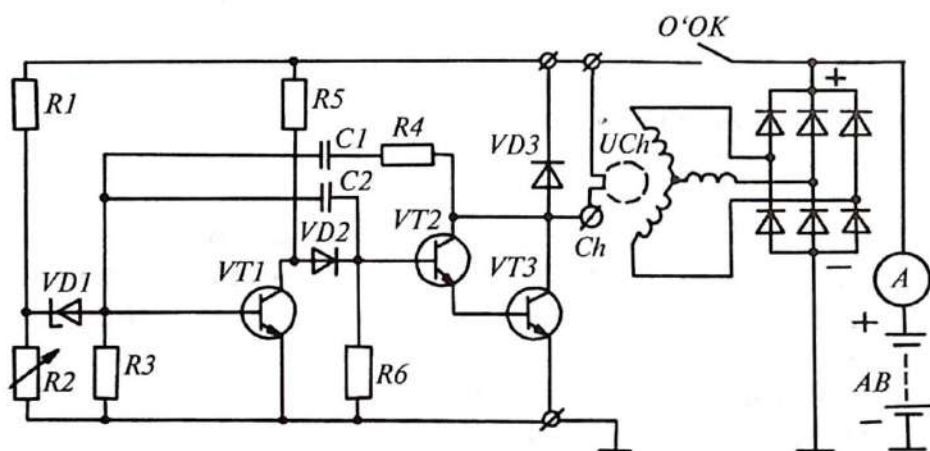
1.35-rasm. Я112 belgili integral kuchlanish rostlagichining chizmasi.
