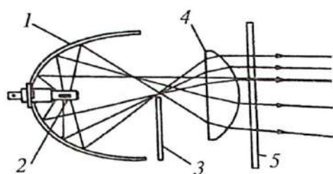
5.8-rasm. Elliptik faraning optik tizimi:
