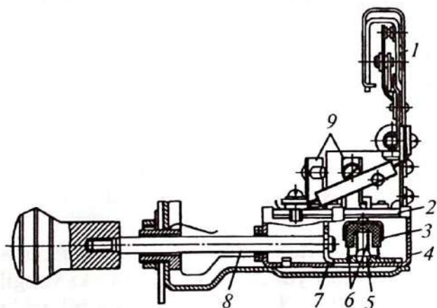
8.1-rasm. Markaziy almashlab ulagich.
