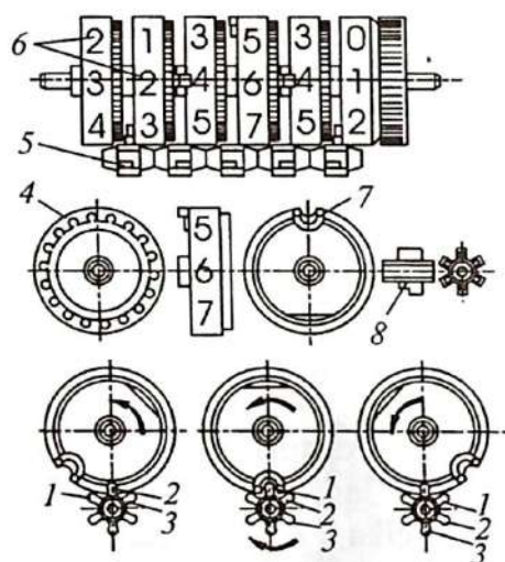
4.13-rasm. Tashqi ilashishli hisoblash mexanizmi.
