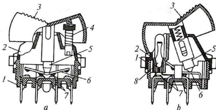
8.2-rasm. Klavishali almashlab ulagichlar:
