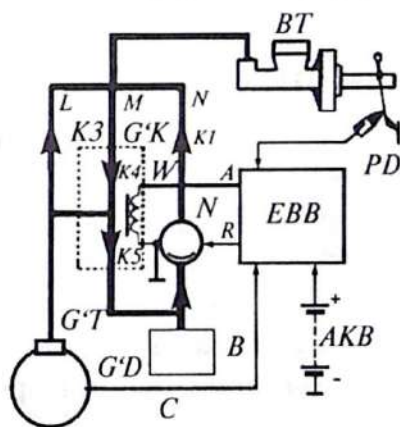
6.12-rasm. ABT tizimining funksional modeli.
