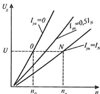
1.22-rasm. O'zgaruvchan tok generatorining ishchi tavsifnomasi.
