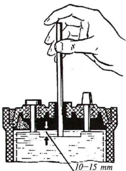
1.12-rasm. Elektrolit sathini o'lchash.
