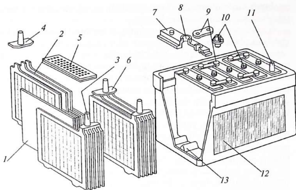
1.1-rasm. Alohida qopqoqli akkumulator batareyasi:
