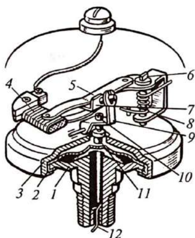
4.5-rasm. Logometrik manometrning reostatli datchigi.
