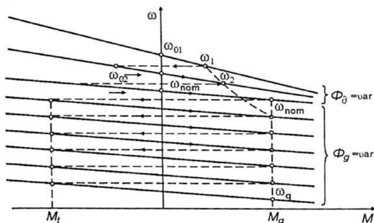
3.4- rasm. Generator-dvigatel tizimini tormozlashdagi mexanik tavsiflar.
