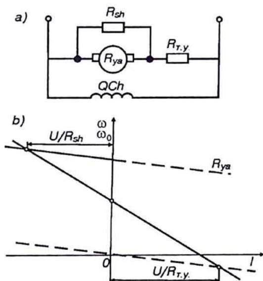
2.11- rasm. Mustaqil qo'zg'atishli dvigatelning yakori shuntlangandagi ulanish sxemasi ( a ) va mexanik tavsiflari ( b ).
