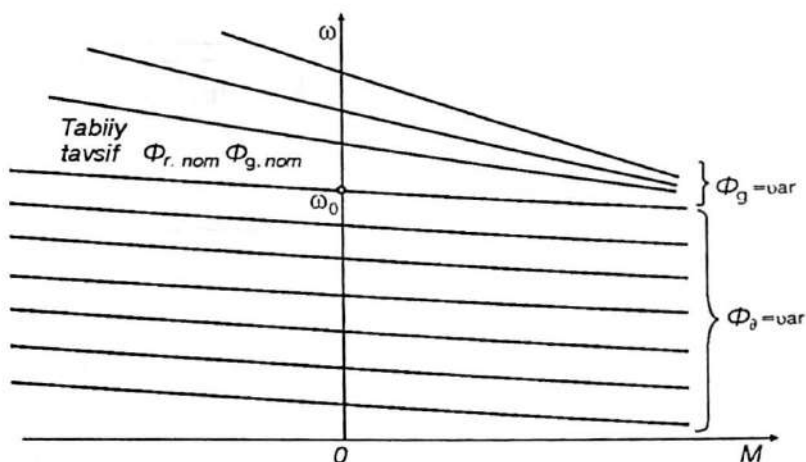
3.2- rasm. Generator-dvigatel tizimining mexanik tavsiflari.
