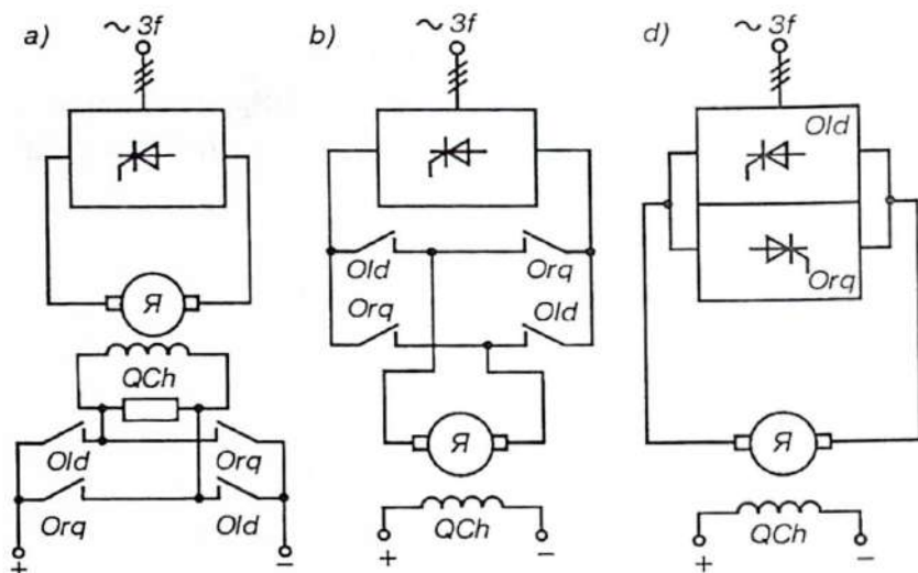
3.9- rasm. BO'-D tizimida reverslashning prinsipial sxemasi:
