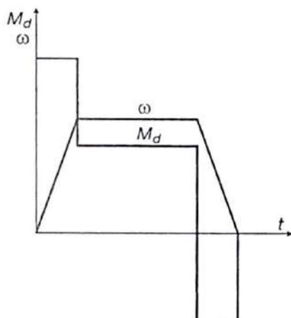
7.1- rasm. Elektr yuritmaning yuklanish diagrammasi.
