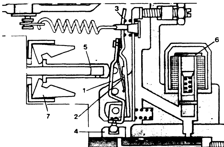
2.99-rasm. Regulatorning to'xtatilishi.
