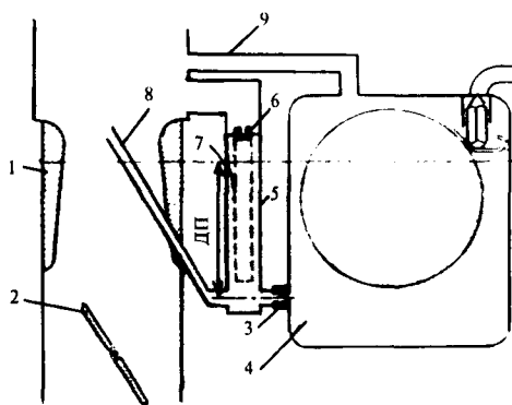
2.50-rasm. Bosh dozlovchi qurilma
