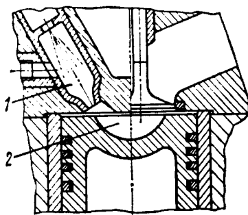
2.75-rasm. Old kamera turli ajratilgan yonish kamerasi:
