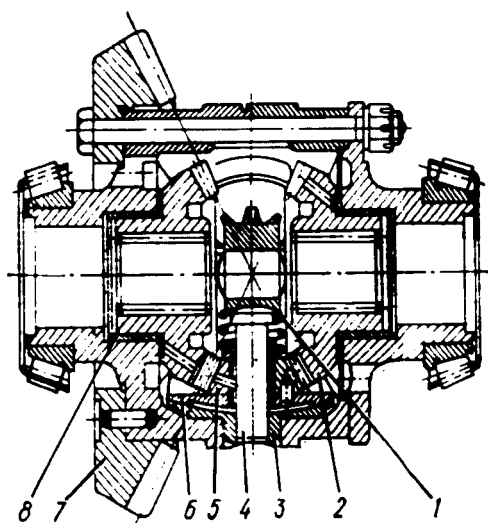
3.46-rasm. MAZ-500
