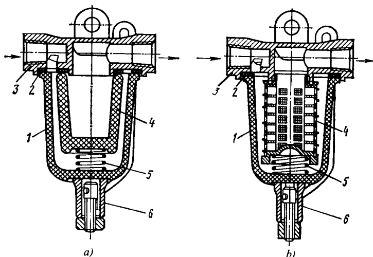
2.66-rasm. Mayin tozalash yonilg'i filtrlari keramika (a) va to'rtli (b) filtrllovchi elementli:
