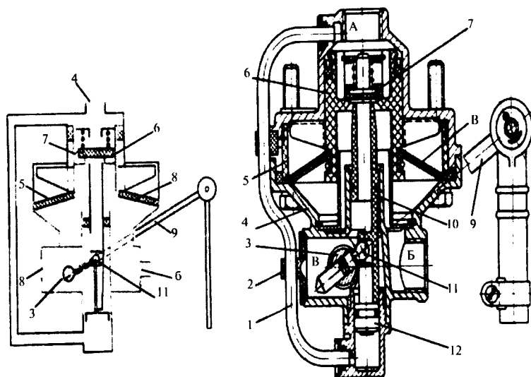
1-trubka; 2-klapan; 3-val; 4-korpus; 5-moslama; 6-porshen; 7-klapan; 8-membrana; 9-richag; 10-chiqarish egari; 11-sharli tayanch; 12-porshen
